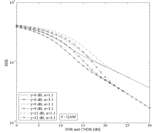
Figure 1: BER estimation for the 4-QAM OFDM system.
