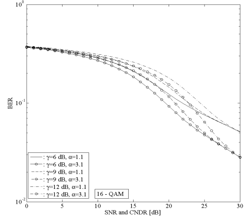
Figure 2: BER estimation for the 16-QAM OFDM system.
