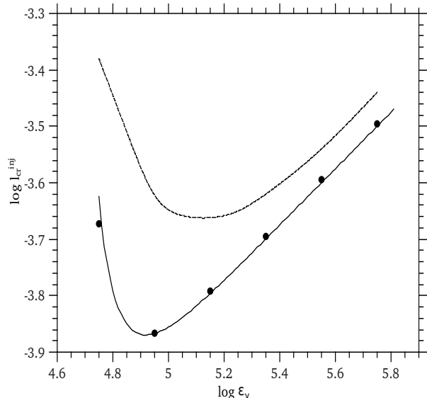
Fig. 3. Critical \gamma -ray compactness as a function of \epsilon_\gamma when (i) \sigma_{\gamma\gamma} and synchrotron emissivity are approximated by a \Theta - and a \delta -function respectively and (ii) when for both quantities the full expressions are used. For the first case the numerical result (points) and the analytical one given by eq.(34) (solid line) are shown. The full problem can only be treated numerically and the corresponding result is shown with a dashed line. The size of the source is R = 3 \times 10^{16} cm and the magnetic field strength B = 3.57 G.
