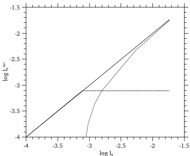
Fig. 4. Plot of the compactness of emerging hard l_\gamma^h (dashed), soft l_\gamma^s (dotted), and total radiated luminosity l_\gamma^{out} (full line) as a function of the injected compactness l_\gamma^{inj} . The \gamma -rays are assumed to be monoenergetic, injected at energy \epsilon_\gamma = 2.3 \times 10^4 . The size of the source is R = 3 \times 10^{16} cm, while the magnetic field strength is B = 40 G. The emerging soft radiation is a result of the self-quenching of the system.
