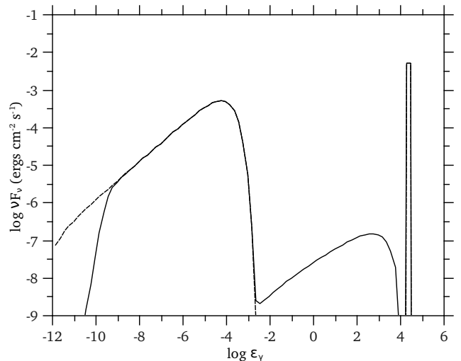
Fig. 5. Multiwavelength spectrum for a choice of l_\gamma^{inj} such that l_\gamma^s = l_\gamma^h . The other parameters are the same as in Fig. 4. Full line corresponds to the case where all relevant radiative processes were taken into account, while the dashed line corresponds to the case where only the two ‘core’ processes were considered, i.e., synchrotron and \gamma\gamma interactions.
