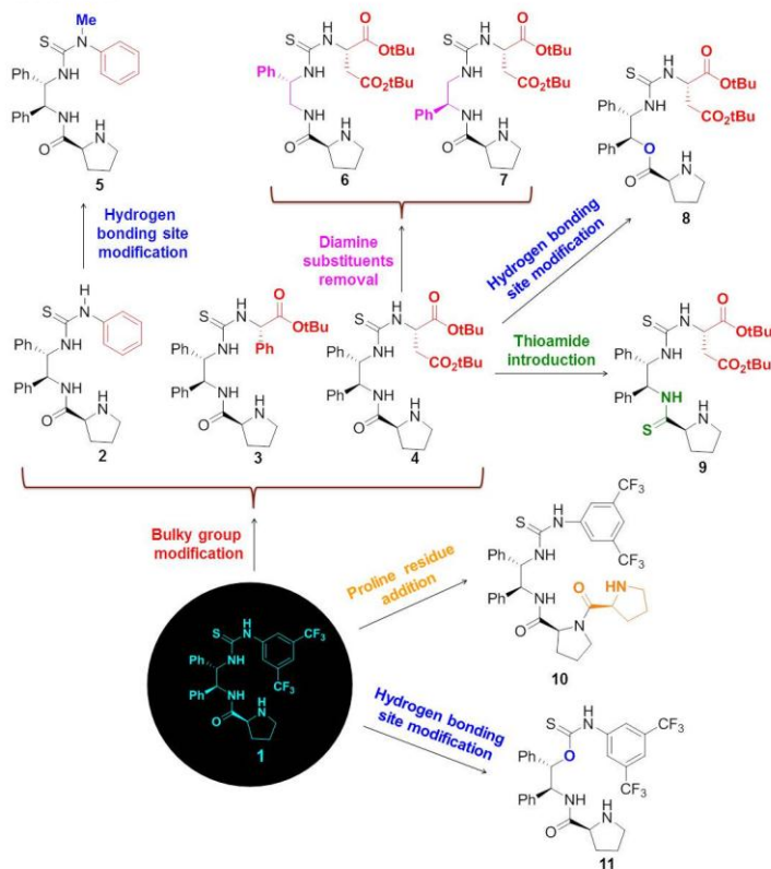
Scheme 1. Modifications of the prolinamide catalyst 1 in order to achieve optimum efficacy. 3
