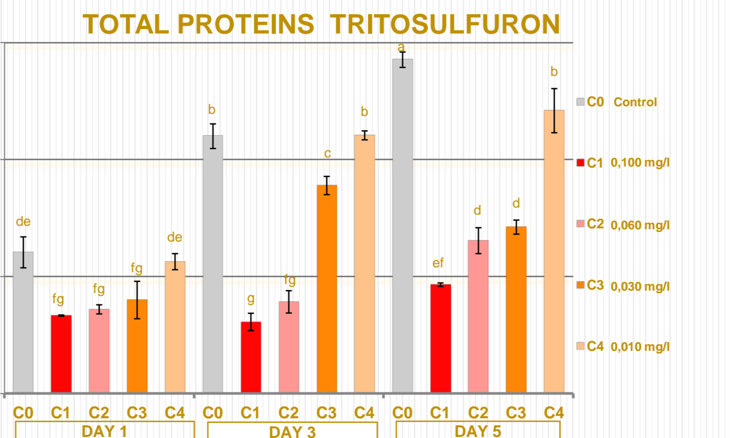
Figure 8: Total proteins in mg per gram fresh weight (mg/gFW) after tritosulfuron exposure in day1, day 3 and day 5 of the trial in control and the 4 concentrations tested. Values are means ± SE from three replicates. Different letters indicate significantly different values at P<1%.
