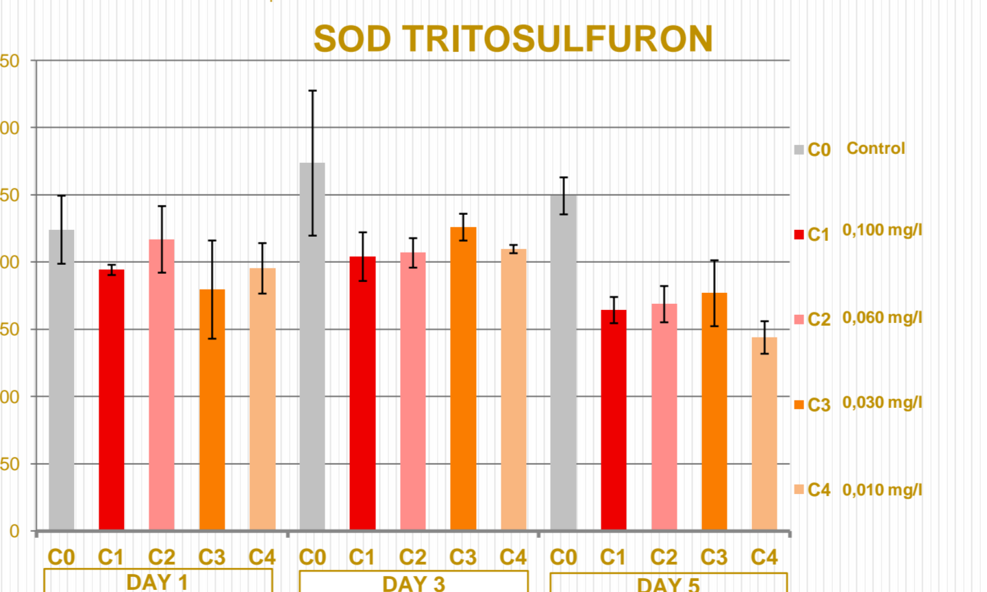
Figure 7: The activity of SOD in mol substrate converted to product per minute (U or units) per gram fresh weight (mol/g FW) after tritosulfuron exposure in day1, day 3 and day 5 of the trial in control and the 4 concentrations tested. Values are means ± SE from three replicates.
