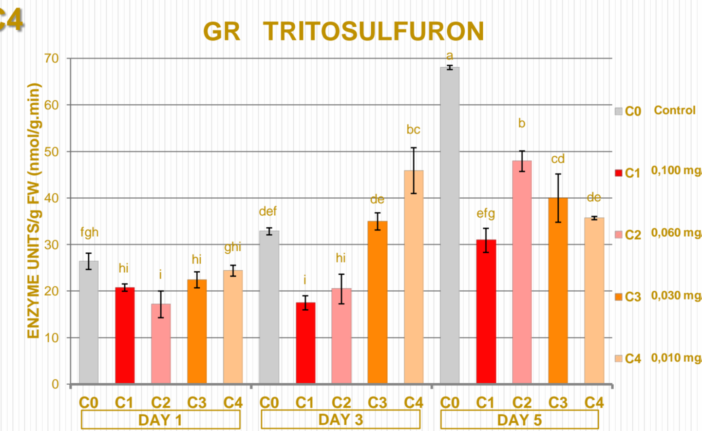
Figure 5: The activity of GR in nmol substrate converted to product per minute (U or units) per gram fresh weight (nmol/g FW) after tritosulfuron exposure in day1, day 3 and day 5 of the trial in control and the 4 concentrations tested. Values are means ± SE from three replicates. Different letters indicate significantly different values at P<1%.
