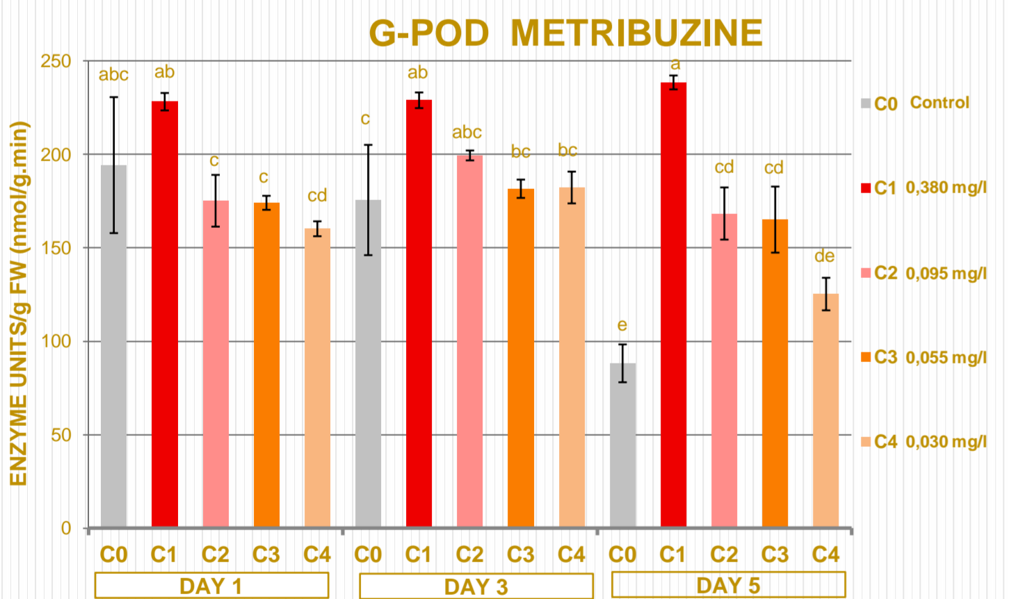
Figure 2: The activity of G-POD in nmol substrate converted to product per minute (U or units) per gram fresh weight (nmol/g FW) after metribuzine exposure in day1, day 3 and day 5 of the trial in control and the 4 concentrations tested. Values are means ± SE from three replicates. Different letters indicate significantly different values at P<0.05.
