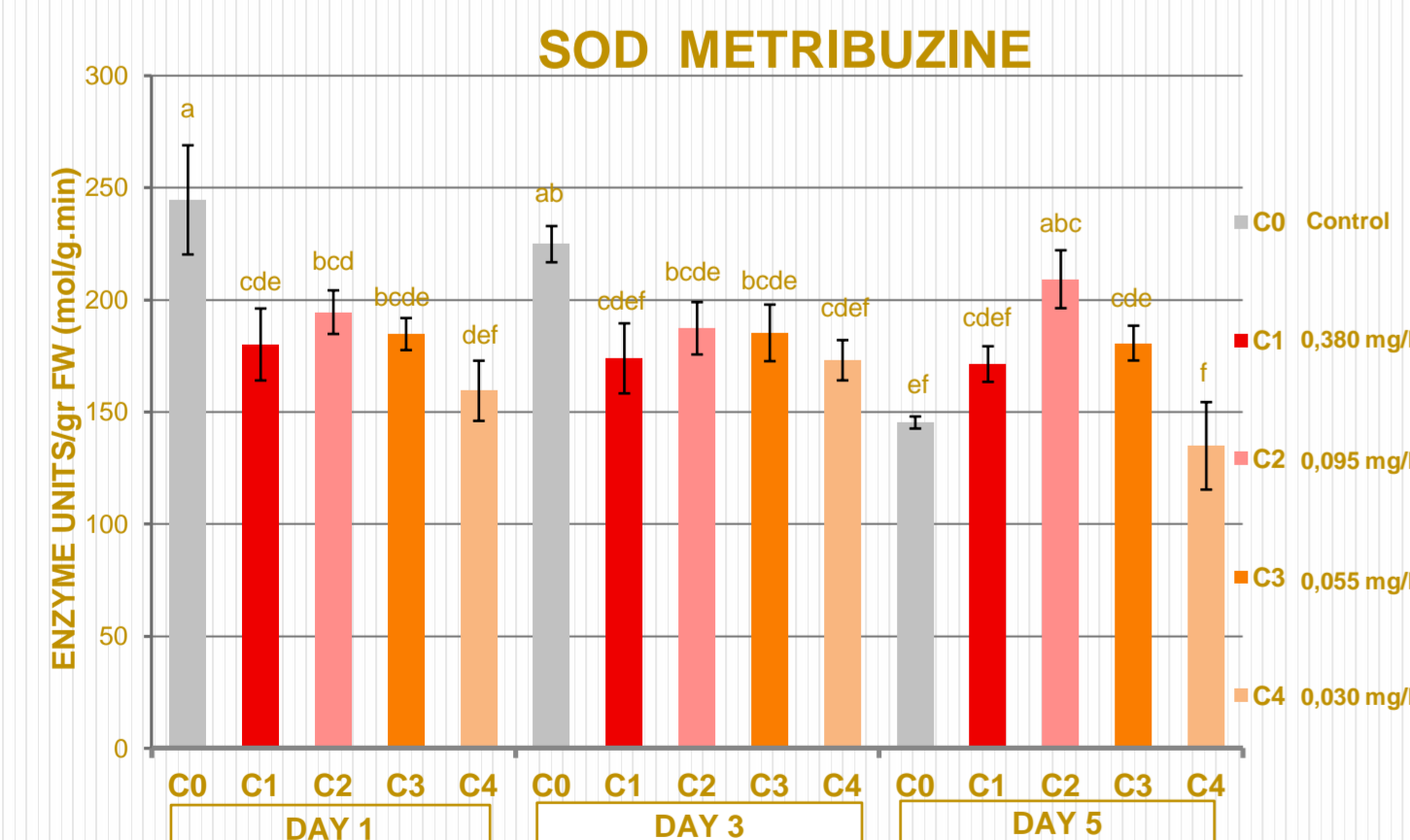
Figure 3: The activity of SOD in mol substrate converted to product per minute (U or units) per gram fresh weight (mol/g FW) after metribuzine exposure in day1, day 3 and day 5 of the trial in control and the 4 concentrations tested. Values are means ± SE from three replicates. Different letters indicate significantly different values at P<0.01.
