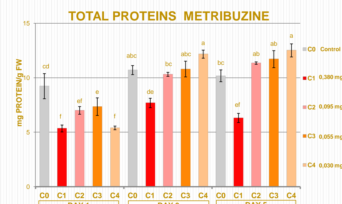
Figure 4: Total proteins in mg per gram fresh weight (mg/gFW) after metribuzine exposure in day1, day 3 and day 5 of the trial in control and the 4 concentrations tested. Values are means ± SE from three replicates. Different letters indicate significantly different values at P<1%.
