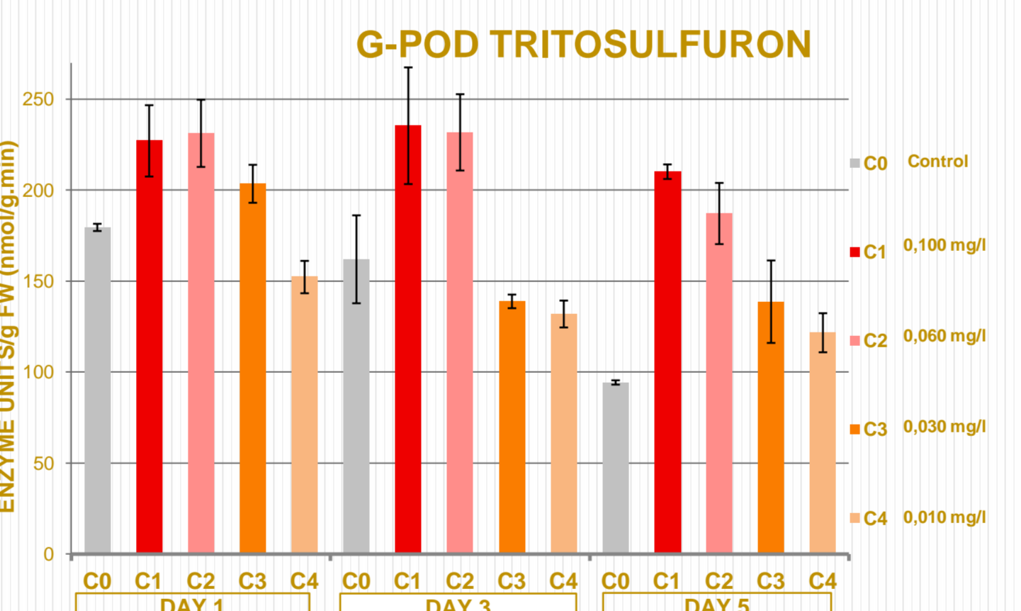
Figure 6: The activity of G-POD in nmol substrate converted to product per minute (U or units) per gram fresh weight (nmol/g FW) after tritosulfuron exposure in day1, day 3 and day 5 of the trial in control and the 4 concentrations tested. Values are means ± SE from three replicates.
