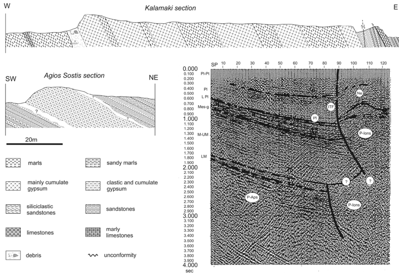
Figure 2. Kalamaki and Agios Sostis sections. Modified seismic profile of the Fig. 1 seismic line (initial interpretation by Marinescu; in Nikolaou 1986): PI-Pt: Pliocene-Pleistocene, PI: Pliocene, LPI: Lower Pliocene, Mes-g: Messinian Gypsum, M-UM: Middle-Upper Miocene, LM: Lower Miocene, P-Aps: Pre-Neogene sequence of Pre-Apulia zone, P-Ions: Pre-Neogene sequence of Ionian zone–Triassic evaporites, ITF: Ionian Thrust Front, Ne: Undifferentiated Neogene, SP: Shot point, sec: Time in seconds.
