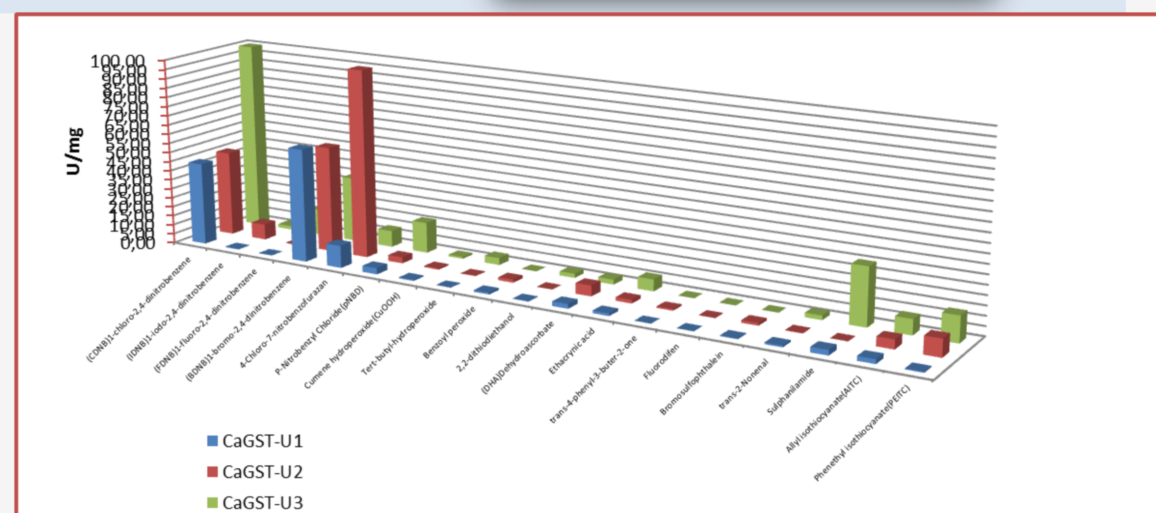
Fig 2: Substrate specificity for purified recombinant CaGST-U1, CaGST-U2, CaGST-U3, towards 19 different electrophilic substrates. Enzyme assays were carried out under standard conditions. Results represent the means of triplicate determinations.
