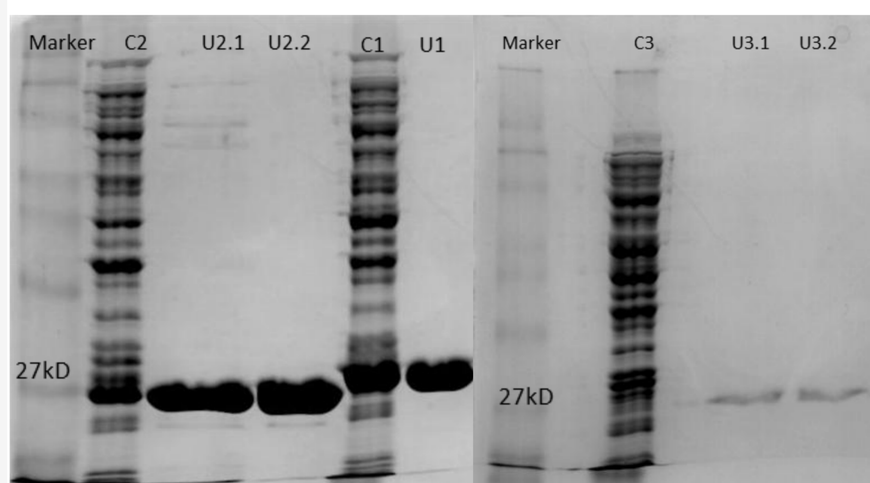
Fig 1: SDS-PAGE analysis of purified CaGST-U1, CaGST-U2, CaGST-U3. Elution was carried out using GSH (10 mM).M protein markers, lane C1,C2,C3 crude extract, lanes U1-U3 eluted fractions of the affinity column.
