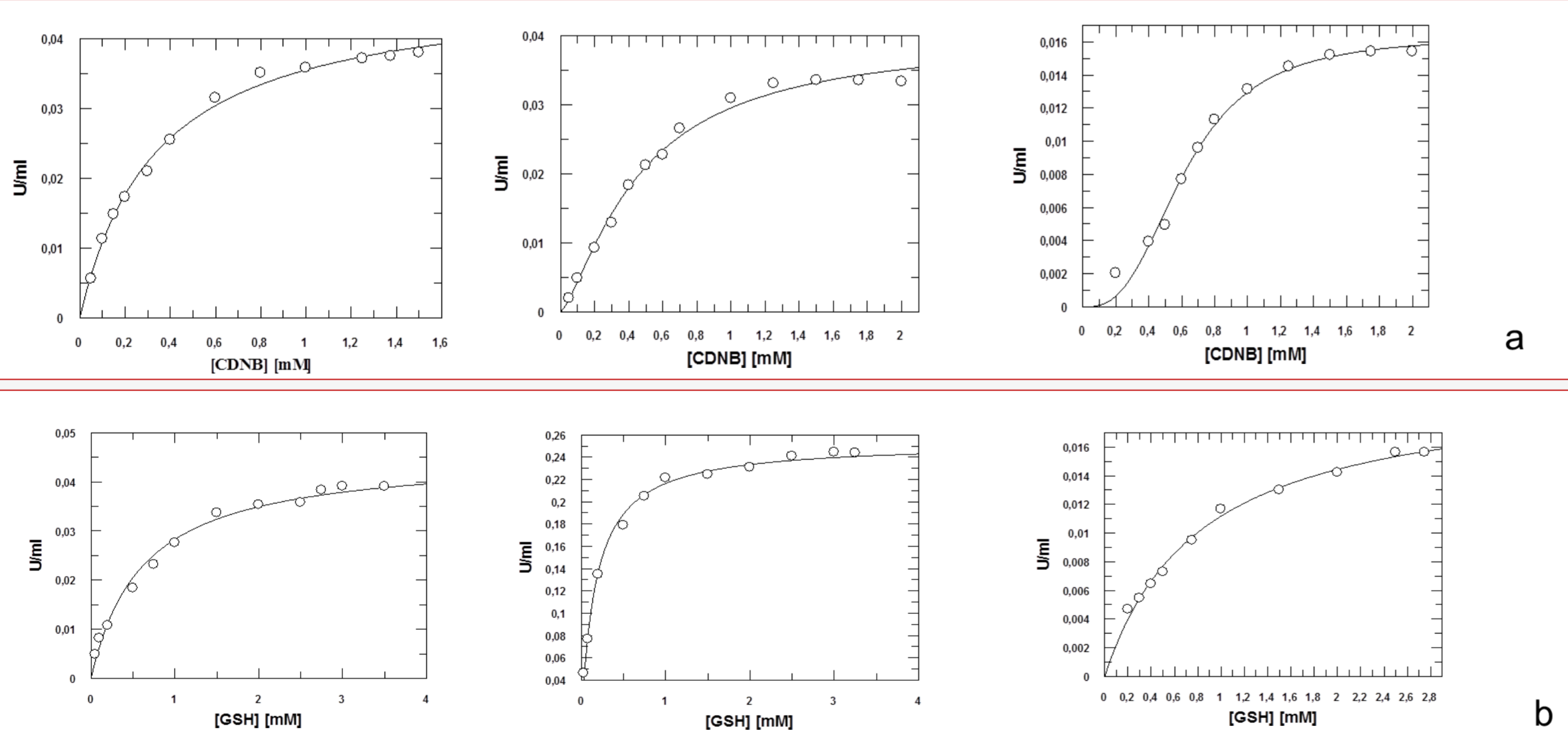
Fig 3: Kinetic analysis of CaGST-U1, CaGST-U2, CaGST-U3 using the CDNB as a variable substrate (a) and GSH at a fixed concentration. Kinetic analysis of CaGST-U1, CaGST-U2, CaGST-U3 using the GSH as variable substrate (b) and CDNB at a fixed concentration. Experiments were performed in triplicate, and lines were those calculated by least-squares regression analysis.
