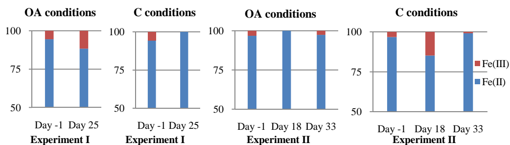
Figure 1 - Fe species ratios in % (Fe(II)/Fetotal and Fe(III)/Fetotal) variation during the two experiments
