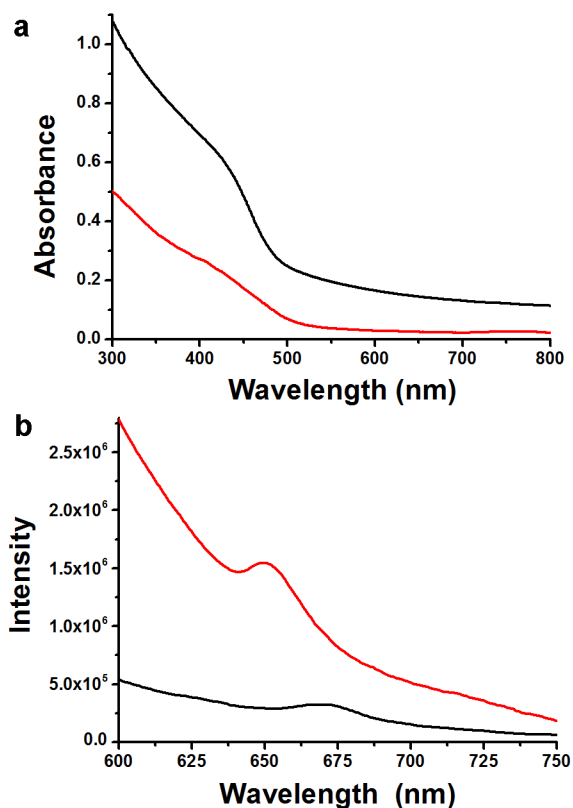
Figure 2. UV-Vis absorption (a) and photoluminescence (b) spectra of CdS•PI- b -PAA/graphene nanoensemble (black) and reference CdS•PI- b -PAA (red), respectively, obtained in NMP:H 2 O (1:1). The excitation wavelength was 400 nm, and the concentrations were adjusted so that CdS in the two samples exhibited equal absorbance at the excitation wavelength.
