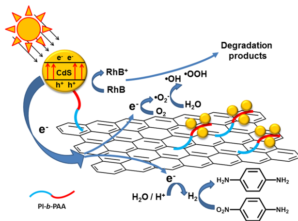
Figure 5. Illustration of the proposed mechanism for the photocatalytic processes responsible for the water splitting and H 2 production (under nitrogen) and the degradation of aqueous RhB (under air) by visible light irradiation of CdS•PI- b -PAA/graphene ensemble.
