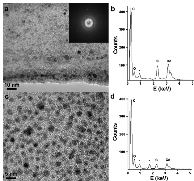
Figure 1. HR-TEM images [(a), (c)] and EDX spectra [(b), (d)] of CdS•PI- b -PAA/graphene ensemble and reference CdS•PI- b -PAA material, respectively. In the EDX spectra [(b), (d)], stars denote the elements Cu and Si, which are detected because of their presence in the microscope equipment, sample holder, and crystal detector. The inset in HR-TEM image of CdS•PI- b -PAA/graphene ensemble shows the FFT from the specific selected area electron diffraction.
