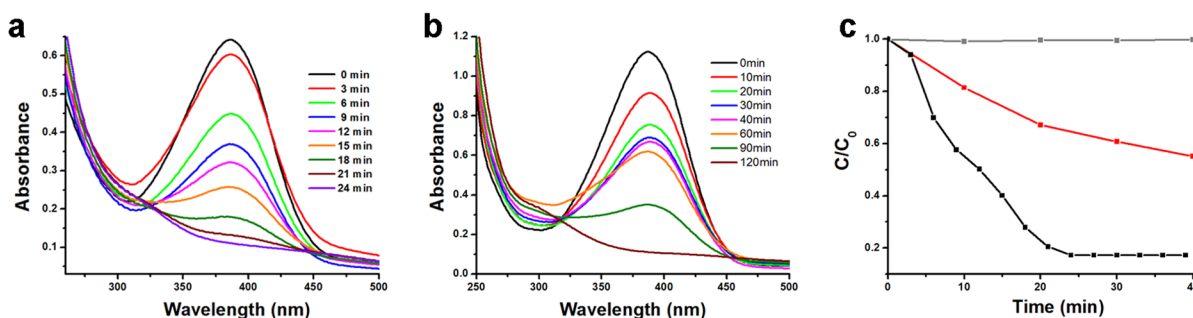
Figure 3. UV-Vis absorption spectra of 4-nitroaniline over (a) CdS•PI- b -PAA/graphene, and (b) CdS•PI- b -PAA, under visible light irradiation, in the presence of ammonium formate as sacrificial agent and N 2 purge. (c) Photocatalytic performance of CdS•PI- b -PAA/graphene (black), reference CdS•PI- b -PAA (red) and exfoliated graphene (grey) in the reduction of aqueous 4-nitroaniline under visible light irradiation in the presence of N 2 .
