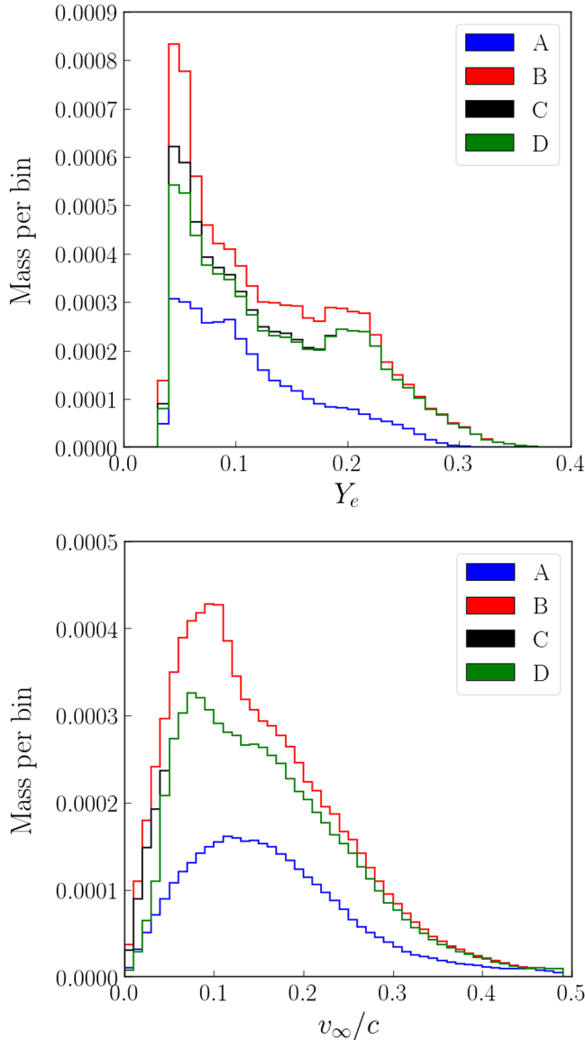
FIG. 1. Predicted mass of unbound matter as a function of Y_e (top) and of the asymptotic speed v_\infty (bottom) in a NSNS simulation for our four outflow models.
