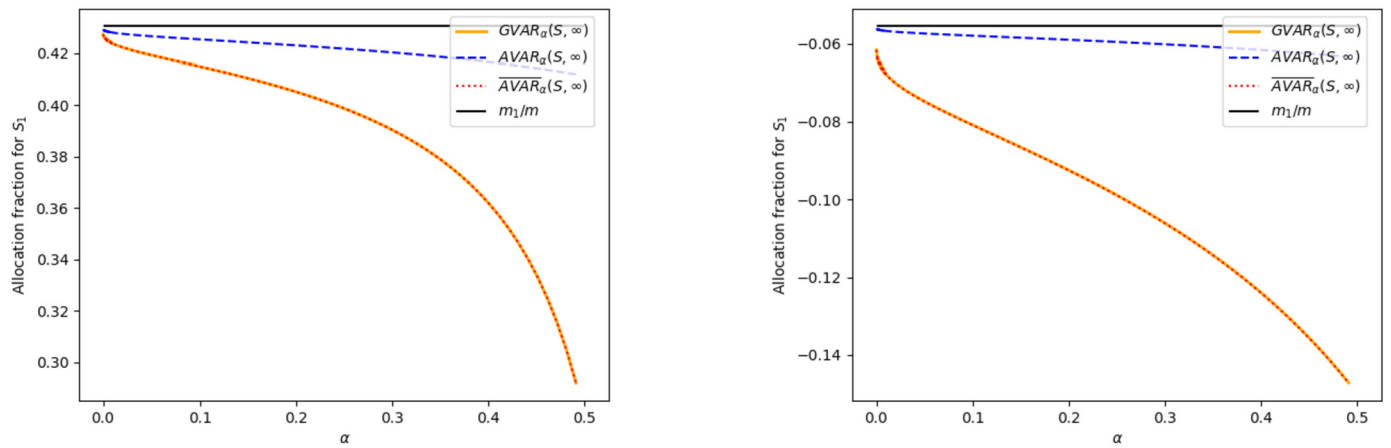
Fig. 4. Allocation fractions of the first risk process AVAR_\alpha^\alpha(S, \infty)/VaR^\alpha(S, \infty) , \overline{AVAR}_\alpha^\alpha(S, \infty)/VaR^\alpha(S, \infty) and GVAR_\alpha^\alpha(S, \infty)/VaR^\alpha(S, \infty) as a function of \alpha . Left panel: \beta_1 = 0.85, \beta_2 = 0.95, \theta = 1, r_1 = 1.5, r_2 = 1.5 . Right panel: \beta_1 = 0.8, \beta_2 = 1, \theta = 1, r_1 = 1, r_2 = 1 .
