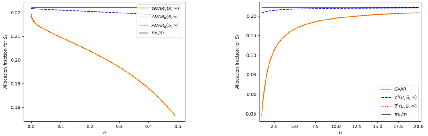
Fig. 3. Allocation fractions of the first risk process as a function of \alpha and u for \beta_1 = 0.85, \beta_2 = 0.95, \theta = 1, r_1 = 1, r_2 = 1 . The left panel: GVAR_\alpha^\alpha(S, \infty)/VaR^\alpha(S, \infty) , \overline{VaR}^\alpha(S, \infty)/VaR^\alpha(S, \infty) , and AVAR_\alpha^\alpha(S, \infty)/VaR^\alpha(S, \infty) as functions of \alpha . Right panel: c_1(u, S, \infty) and \bar{c}_1(u, S, \infty) as a function of u .
