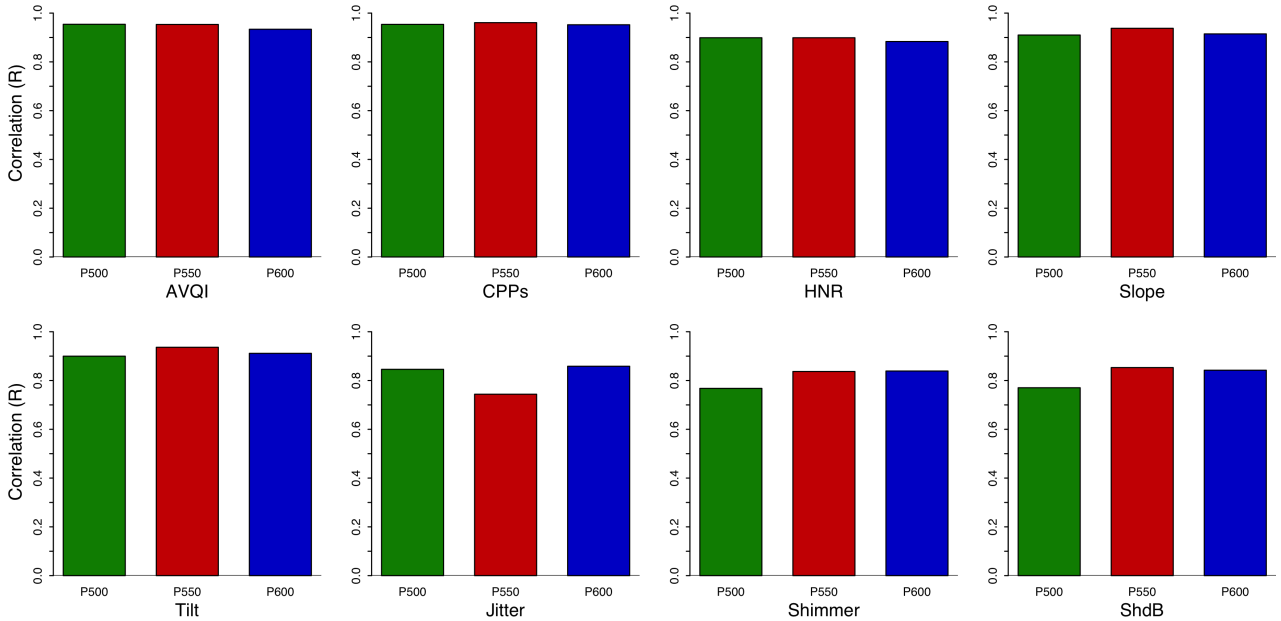
Figure 2: Pearson’s correlation coefficients between Pseudonymized and Original values of parameters. All R: p < 0.001 . P500 (green): \phi = 500 Hz, F_0 = 120 Hz; P550 (red): \phi = 550 Hz, F_0 = 150 Hz; P600 (blue): \phi = 600 Hz, F_0 = 180 Hz. See text.
