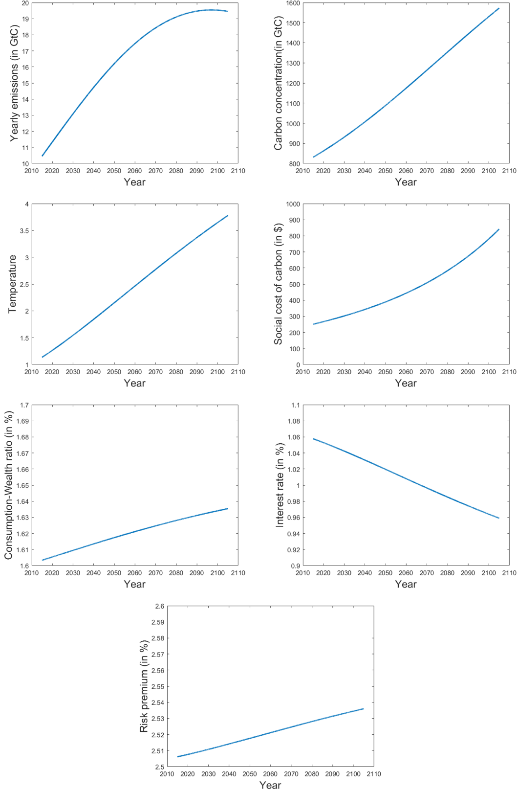
Figure 3.6: The expected paths of emissions, carbon concentration, temperature, social cost of carbon, consumption-wealth ratio, risk-free rate and the risk premium over time.
