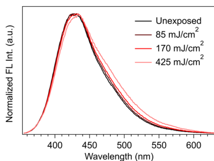
Figure 2. Normalized fluorescence spectra of pristine and EUV-exposed ZrMc–CB films on quartz ( \lambda_{\text{exc}} = 345 nm).
