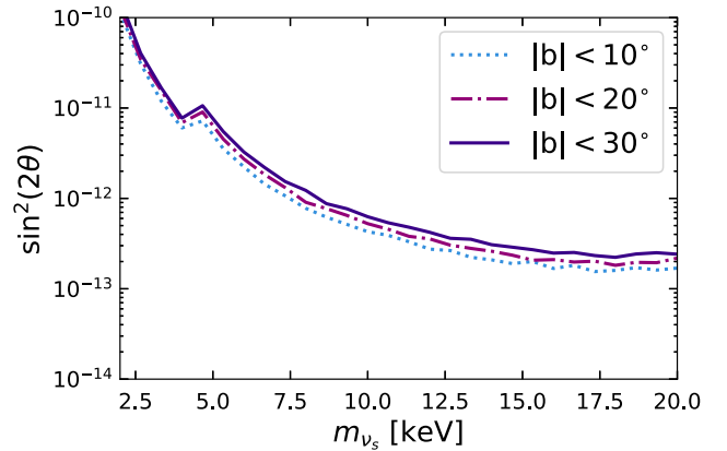
FIG. 4. Sensitivity to the mixing angle, adopting a NFW density profile. The pixels with the following Galactic latitudes are removed: |b| < 10^\circ (dotted), |b| < 20^\circ (dot-dashed), and |b| < 30^\circ (solid).
