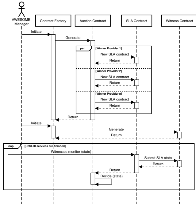
Figure 4: The Sequence Diagram of the AWESOME Smart Contracts Interactions.
