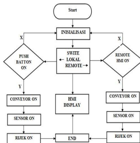
Gambar 3 flowchart
