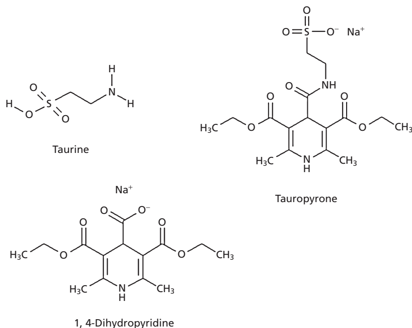
Figure 1 Chemical structures of taurine, tauroprone and the 1,4-dihydropyridine moiety.
