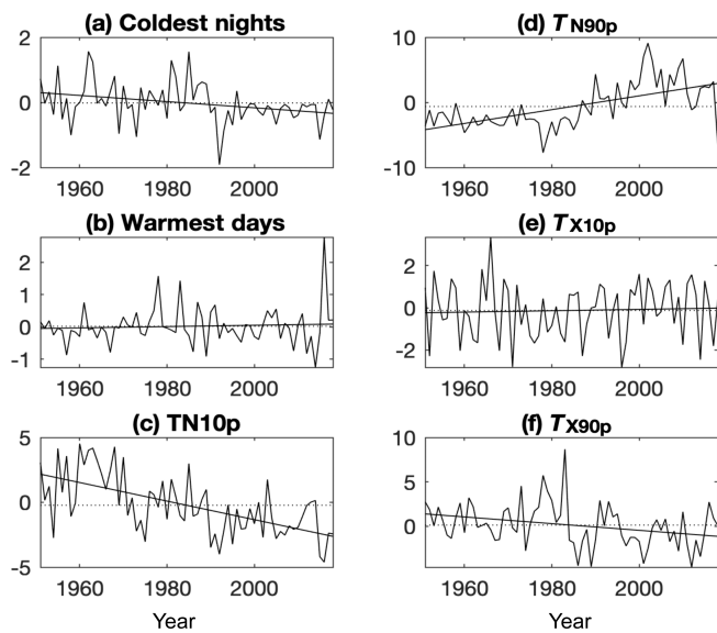
FIGURE 8 Continuation of Figure 7 for (a) coldest nights; (b) hottest days; (c) T_{N10p} ; (d) T_{N90p} ; (e) T_{X10p} ; and (f) T_{X90p} from 1951 to 2018 in the Philippines. Statistically significant trends were observed in the T_{N10p} , T_{N90p} , and coldest nights indices
