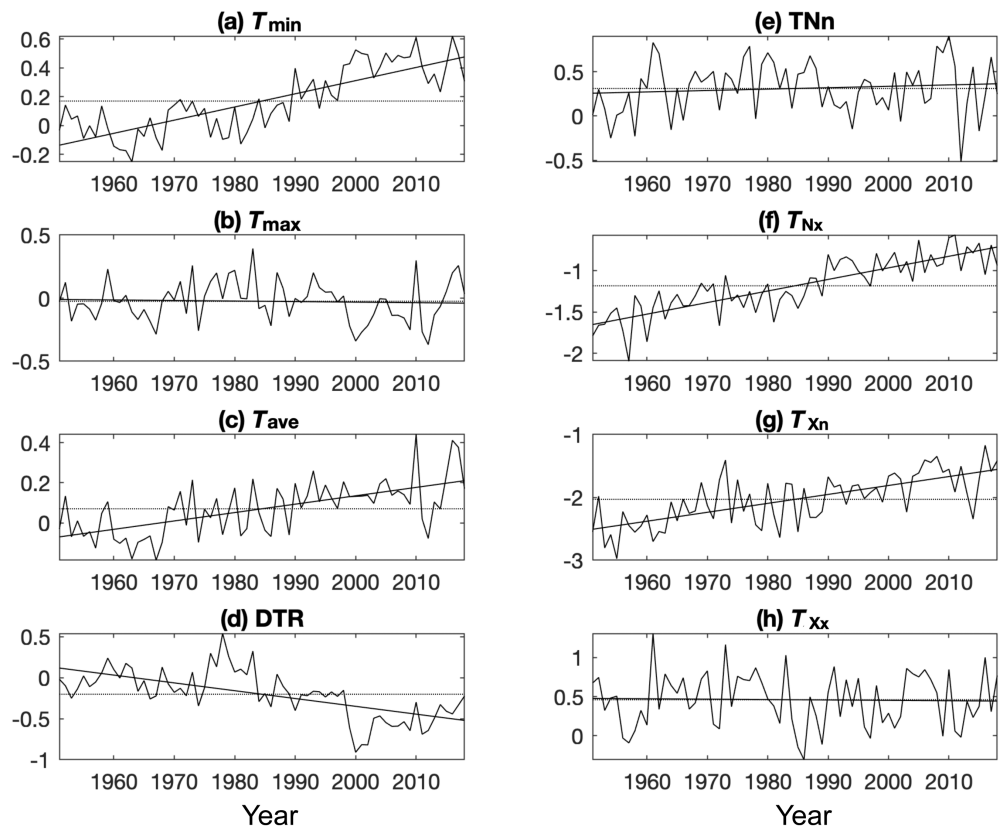
FIGURE 7 Time series of the effect of urbanization on the temperature indices (a) T_{min} ; (b) T_{max} ; (c) T_{ave} ; (d) DTR; (e) T_{Nn} ; (f) T_{Nx} ; (g) T_{Xn} ; and (h) T_{Xx} from 1951 to 2018 in the Philippines. Statistically significant trends at the 95% confidence level were observed for the T_{ave} , T_{min} , DTR, T_{Nx} , and T_{Nn} indices. The horizontal line corresponds to the mean (light colour) and linear trend lines (dark colour)
