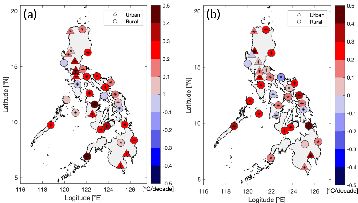
FIGURE 5 Long-term trends of the annual (a) minimum ( T_{min} ) and (b) maximum temperature ( T_{max} ) for the 34 stations in the Philippines from 1951 to 2018. The white star symbol at the centre of the circles denotes that the trends were statistically significant at the 95% confidence level. The shading corresponds to the trends of the urban (triangles) and rural (circles) stations [Colour figure can be viewed at wileyonlinelibrary.com ]
