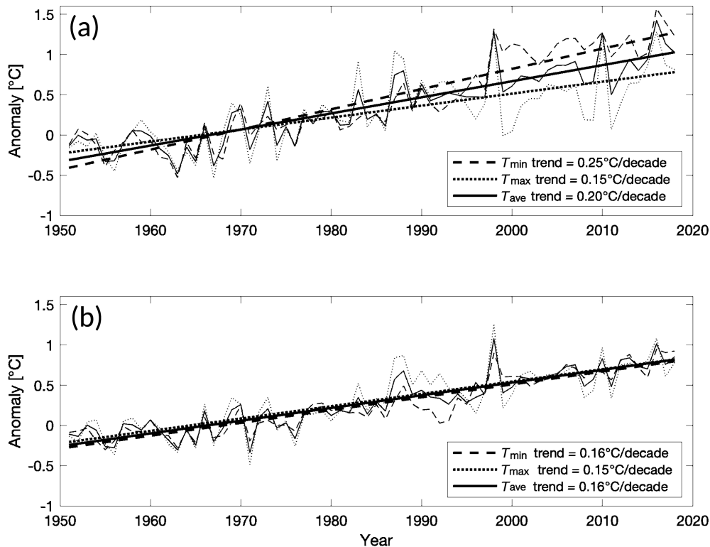
FIGURE 6 Time series of the annual T_{min} , T_{max} , and T_{ave} anomaly for (a) urban and (b) rural stations from 1951 to 2018. The dashed, dotted, and solid lines represent the time series of T_{min} , T_{max} , and T_{ave} , respectively. The thin and thick lines correspond to the annual values and linear trend-line, respectively. All obtained trends were statistically significant at the 95% confidence level
