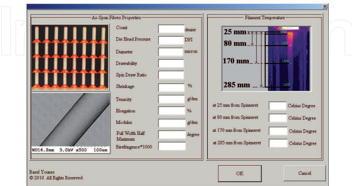
Figure 7. The output interface/window for filament temperature in the machine's cooling window and the fiber's structural, mechanical and physical properties.
