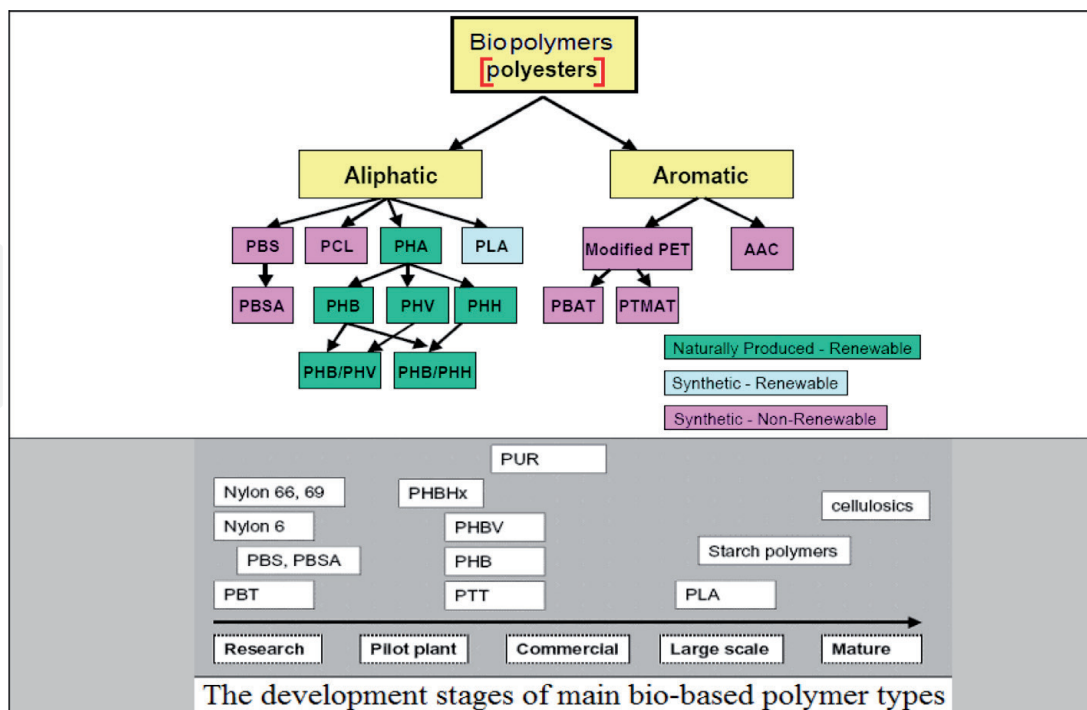
Figure 2. Classification and development of bio-based polymers [26, 27]. PCL – polycaprolactone; PBS – polybutylene succinate; PTT– polytrimethyleneterephthalate; PBBSA – polybutylene succinate adipate; PHH – polyhydroxyhexanoate; AAC – Aliphatic-Aromatic Co-polyesters; PHV – polyhydroxyvalerate; PET – polyethylene terephthalate; PLA – polylactic acid; PBAT – polybutylene adipate/terephthalate; PHA – polyhydroxyalkanoates; PTMAT– polyethylene adipate/terephthalate; PHB – polyhydroxybutyrate (type of PHA); PBT– polybutylene succinate; PHBV, PHBHx- types of PHA; PUR– polyurethanes.
