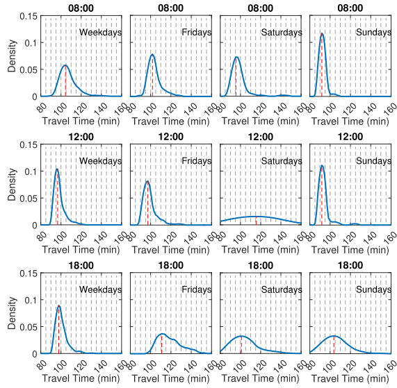
Fig. 2. Kernel density function estimates using (10) of the travel times departed at 08:00, 12:00 and 18:00 (row-wise; top to bottom) for regular weekdays, Fridays, Saturdays, and Sundays (column-wise; left to right) of the Taipei-to-Taichung route.
