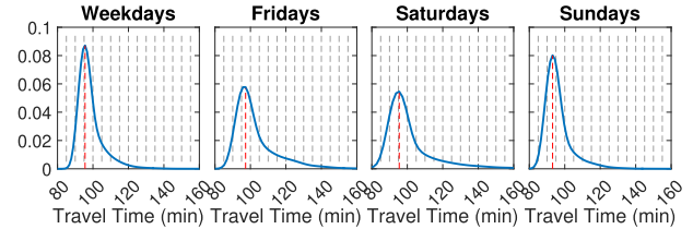
Fig. 4. Estimated mean functions of travel time densities for the Taipei-to-Taichung route.
