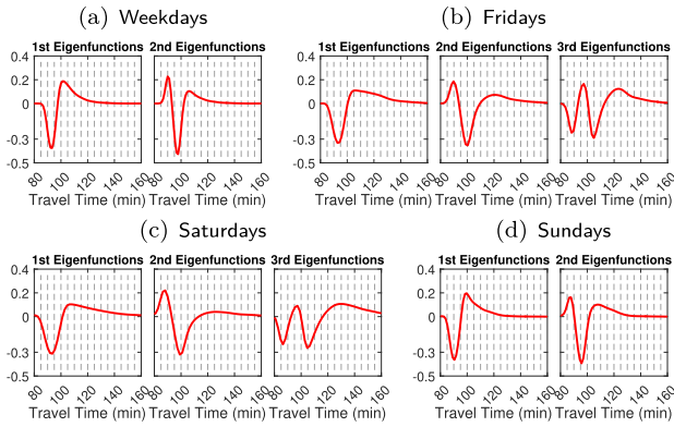
Fig. 6. Estimated eigenfunctions \hat{\phi}_j(t) for travel times of the Taipei-to-Taichung route, with the total number of components selected by the 95% proportion-of-variance-explained criterion using (15).
