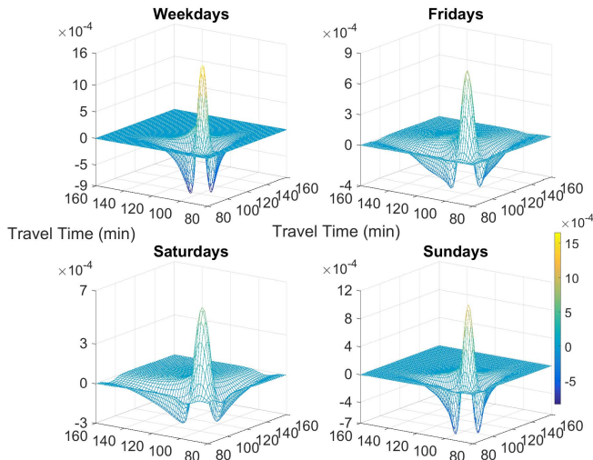
Fig. 5. Estimated covariance functions of travel time densities for the Taipei-to-Taichung route.
