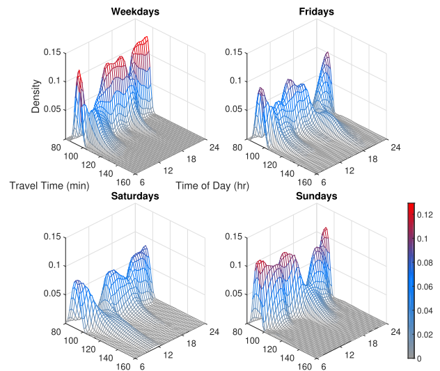
Fig. 8. Fitted travel time density surfaces of the Taipei-to-Taichung route.
