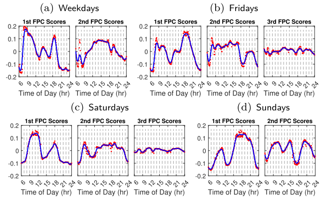
Fig. 7. Estimated conditional expectation \hat{\eta}_j(t) using (13) superimposed on the FPC scores, associated with the eigenfunctions in Fig. 6.
