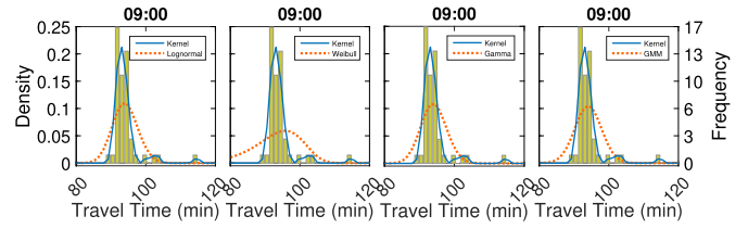
Fig. 3. Comparisons between the fitted parametric density functions (lognormal, Weibull, gamma, and GMM) and the kernel density estimates superimposed on the histograms of the travel times on weekdays departed at 09:00 for the Taipei-to-Taichung route.
