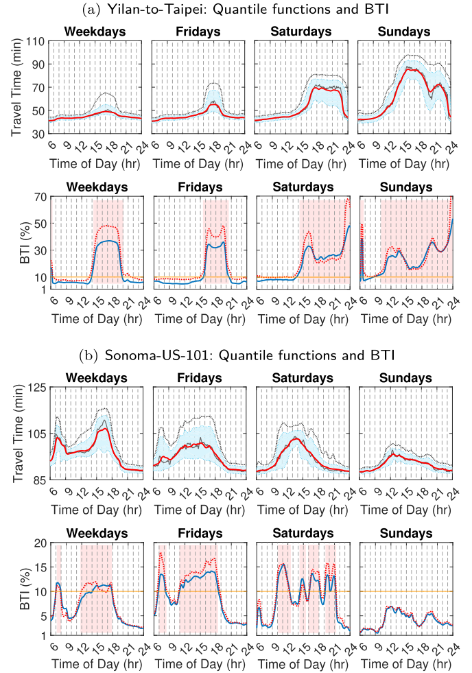
Fig. 10. The estimated quantile functions and the reliability indicators for (a) the Yilan-to-Taipei route and (b) the Sonoma-US-101 route, with a similar layout to Fig. 9.
