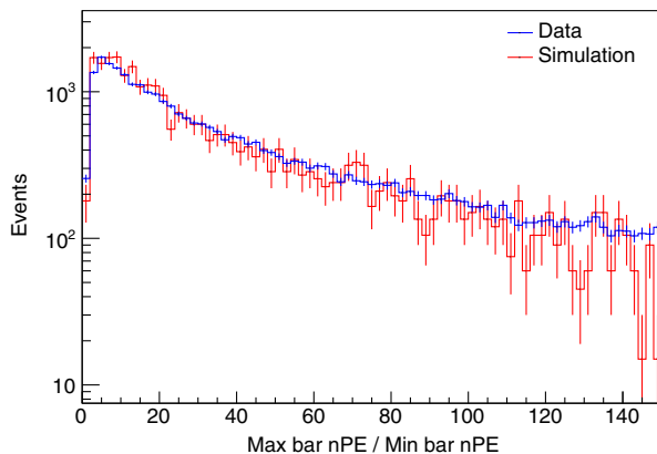
FIG. 5. The ratio of maximum n_{pe} to minimum n_{pe} in cosmic muon events for data (blue) and simulation (red).
