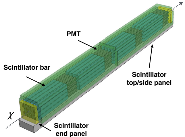
FIG. 1. A diagram of the milliQan Run 3 bar detector components. The scintillator bars are shown in blue connected to PMTs in black. The side and top panels are shown surrounding the bars in transparent green while the end panels are shown in transparent yellow. The PMTs are not shown for the side and top panels. All components are installed on an aluminum tube. The path of a millicharged particle from the IP is shown in gray.
