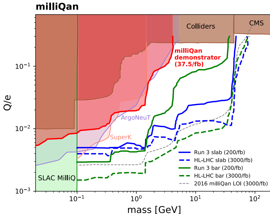
FIG. 7. Expected exclusion at 95% confidence level compared to existing constraints [6–12,15,17,31]. Results from a recent reinterpretation of data collected by the BEBC WA66 beam dump experiment, which provides competitive constraints on millicharge particles with masses below a few GeV, are not shown as only 90% confidence level contours are available [14].
