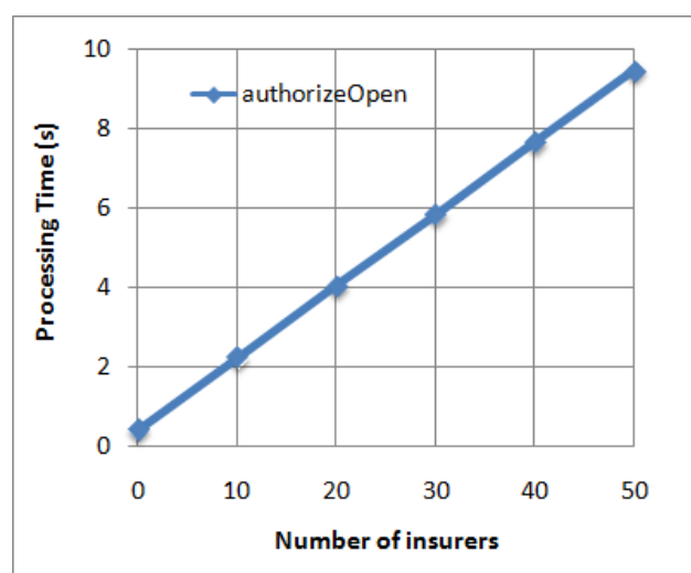
Figure 6. Computational cost for claim authorization by 50 insurers.
