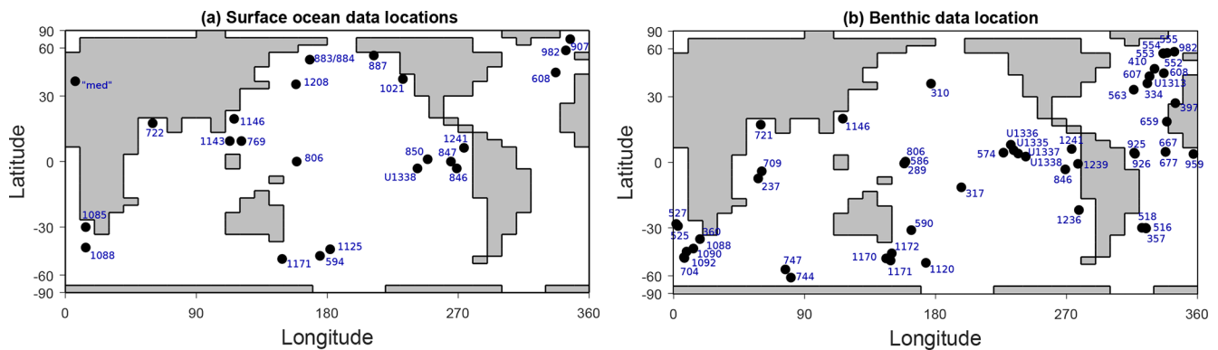
Figure 1. Present-day location of surface ocean temperature data points (a) and benthic \delta^{18}\text{O} and \delta^{13}\text{C} data points (b) collated for this study (the Holocene \delta^{13}\text{C} data set from Peterson et al., 2014, is not plotted).
