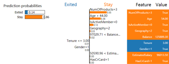
Figure 7: LIME plots.
