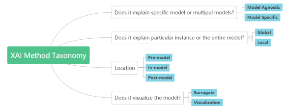
Figure 4: XAI method taxonomy.
