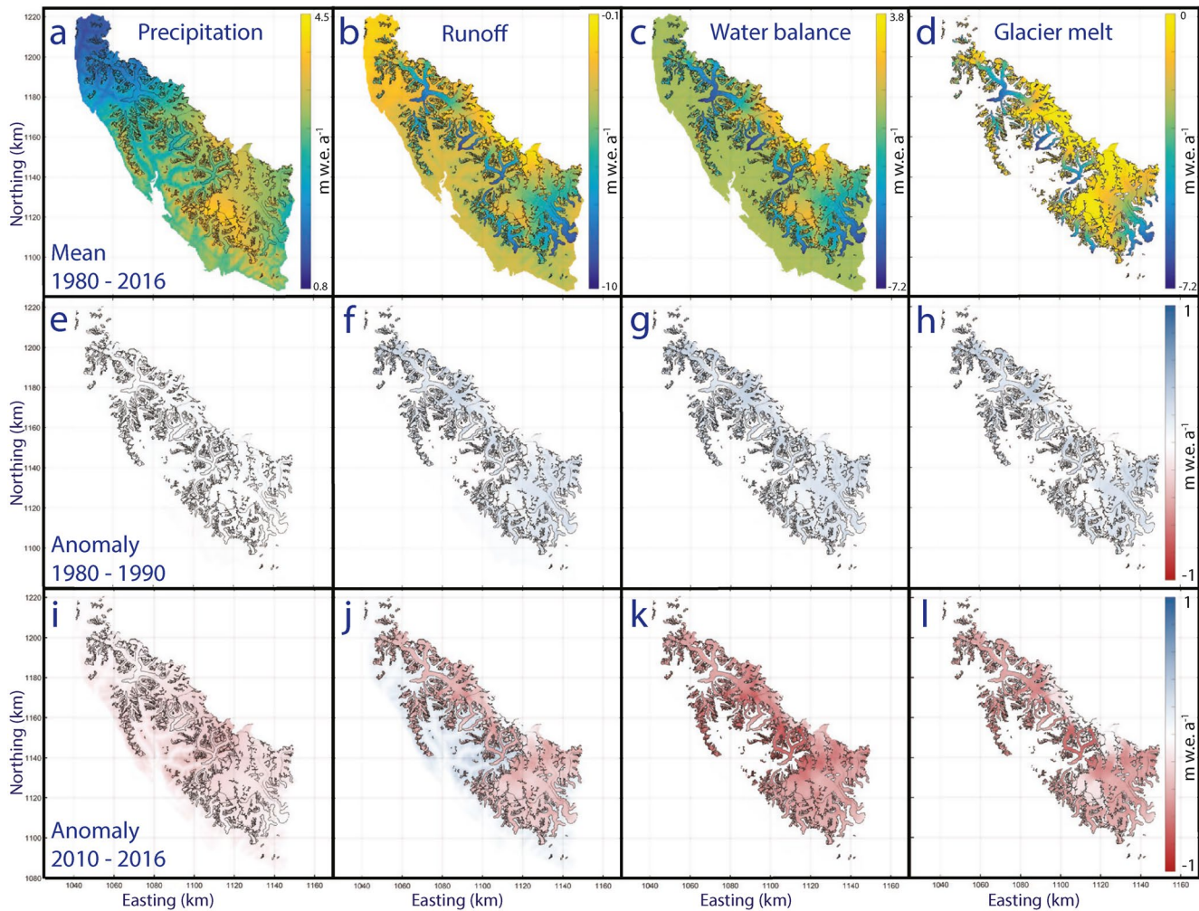
Figure 12. Spatially distributed plots of mean annual rates of precipitation (first column; a, e, and i), total runoff (second column; b, f, and j), water balance (third column; c, g, and k), and glacier ice melt (fourth column; d, h, and l). Figures a–d (first row) display 1980 to 2016 means; note that the scale bars are different for each quantity. Figures e–h (second row) show mean annual anomalies from the 1980 to 2016 mean for the decade 1980 to 1990, while Figures i–l (third row) show anomalies for 2010 to 2016. Figures e–l are displayed using the same color scale. Note the negative sign convention used for glacier ice melt and total runoff in figures f, h, j and l, such that red shading in these quantities indicates a greater (i.e., more negative) volume than the 1980 to 2016 mean.
