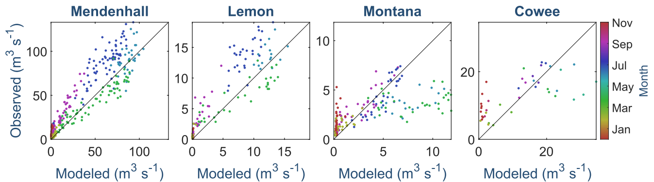
Figure 4. Mean monthly discharge Q from observations versus model results for four instrumented watersheds in cubic meters per second, as driven with the best fit parameters. Time spans of data availability for each gauge differ, and are listed in Table 1. Solid black lines represent 1:1 lines. Note the differing axis scales.
