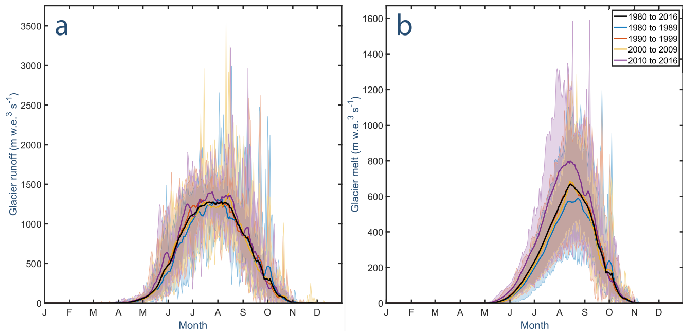
Figure 11. Stacked graphs of modeled output of (a) glacier runoff and (b) glacier ice melt for the coastal domain. Solid colored lines represent the daily mean output for each decade, while shaded regions in matching colors represent the corresponding daily range for all years within the given decade. The solid black line shows the 1980 to 2016 mean. Note that in similar figures (not included) for precipitation, air temperature, water balance, and total runoff variables, interannual variability dominates and obscures any visible shifts in timing or magnitude.
