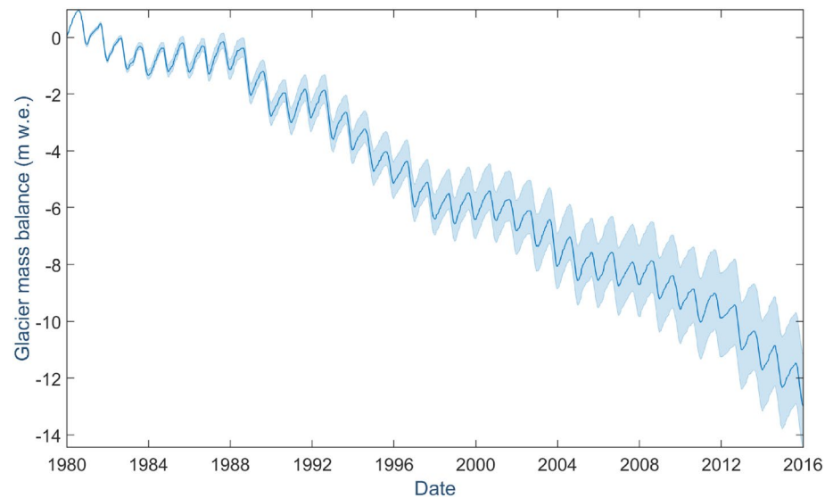
Figure 6. Modeled cumulative glacier-wide specific mass balance for the full model period of October 1, 1980 to September 30, 2016 for all coastal ice of the Juneau Icefield. The upper and lower limits of uncertainty correspond to the ensemble end member simulations, whose trends correspond to the upper and lower limits of uncertainty of the calibrating geodetic mass balance estimate for 2000 to 2016 from (Berthier et al., 2018).
