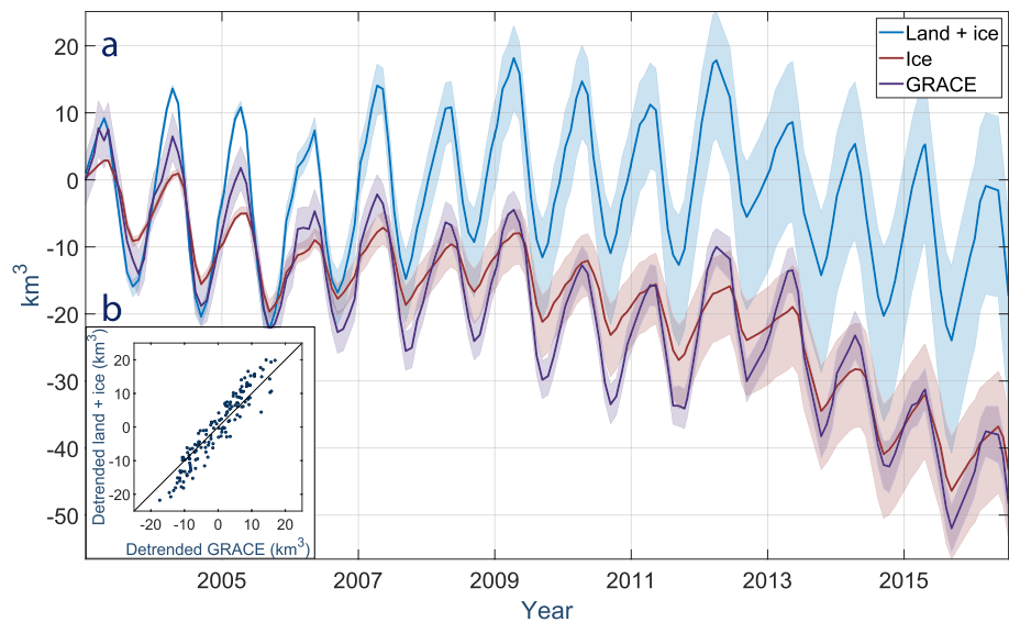
Figure 8. (a) Water balance time series comparing the GRACE solution for 2003 to 2016 (purple) with results derived from SnowModel. Model results for the full GRACE domain (i.e., all land + ice cells together) are shown in blue, while the ice-only area within the GRACE domain (i.e., glacier ice cells alone) is shown in red. (b) Scatter plot comparison of detrended modeled land + ice water balance values versus equivalent from GRACE.
