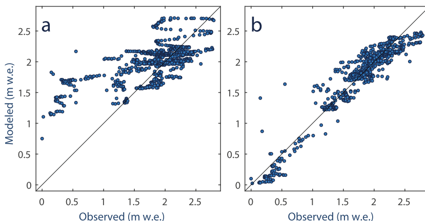
Figure 3. Comparison of observed snow water equivalent (SWE) values from 2013 to 2015 field campaigns conducted as part of this study versus modeled values for the same dates both (a) before, and (b) after the application of the SnowAssim initial calibration routine. Results are shown for the simulation driven with the best fit parameters; other simulations in the final ensemble are similar.
