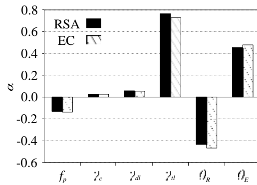
Figure 12. Cosines direction at design point.
