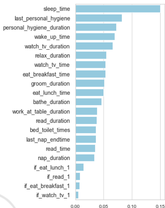
Figure 6: Feature importance of the Random Forest Classifier.
