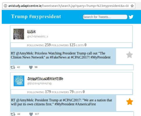
Figure 2: "tweetsearch" interface
