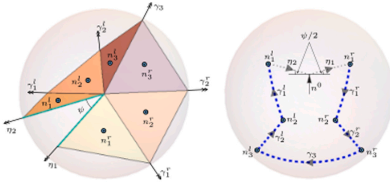
Fig. 4. Gauss map representation of a creased e-cone for m = 3 . Each facet's unit normal (left) is represented by its embedding into the unit sphere S^2 (right). Spherical geodesics connect adjacent facets' normals on S^2 following the folding direction to form a piecewise smooth curve: each portion of the curve has a length equal to the folding angle it represents; and any two portions of the curve form a spherical angle that is equal to the solid angle made by the respective folding lines they represent (which in general is not equal to the panels' subtended angle \alpha_m unless \phi = 0 —in the absence of any stretching).
