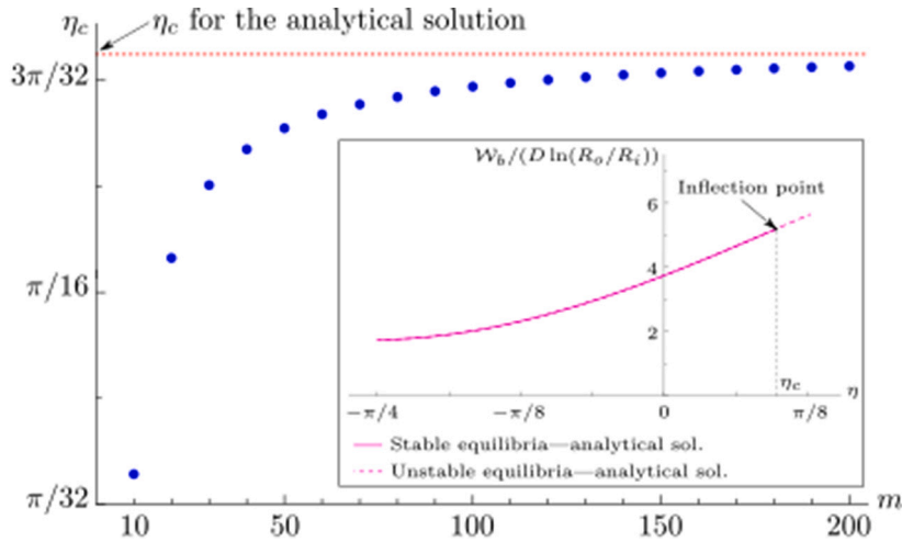
Fig. 6. The onset of instability for the e-cone’s symmetric creased configurations approaches that of the analytical smooth solution (Sadik and Dias, 2021) for an increasing discretisation size m . Here, the excess angle \psi is fixed at \pi/5 . In the inset, we see the onset of instability, \eta_c , i.e., the limit between the stable and unstable configurations: it is a point of inflection for the bending energy as a function of the lips rotation \eta .
