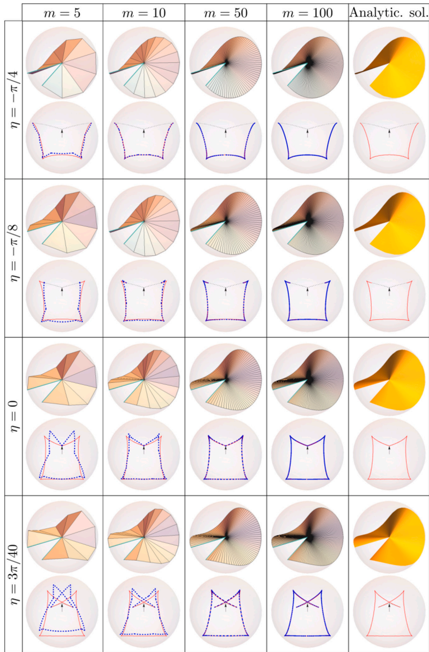
Fig. 5. Gauss map representations of the creased solution for m = 5, 10, 50, \& 100 compared to the analytical results (Sadik and Dias, 2021) for an excess angle of \psi = \pi/5 and lips rotations of \eta = -\pi/4, -\pi/8, 0, \& 3\pi/40 . The creased solution's Gauss maps quickly approach the corresponding analytical solution, even for a relatively small discretisation size, m .
