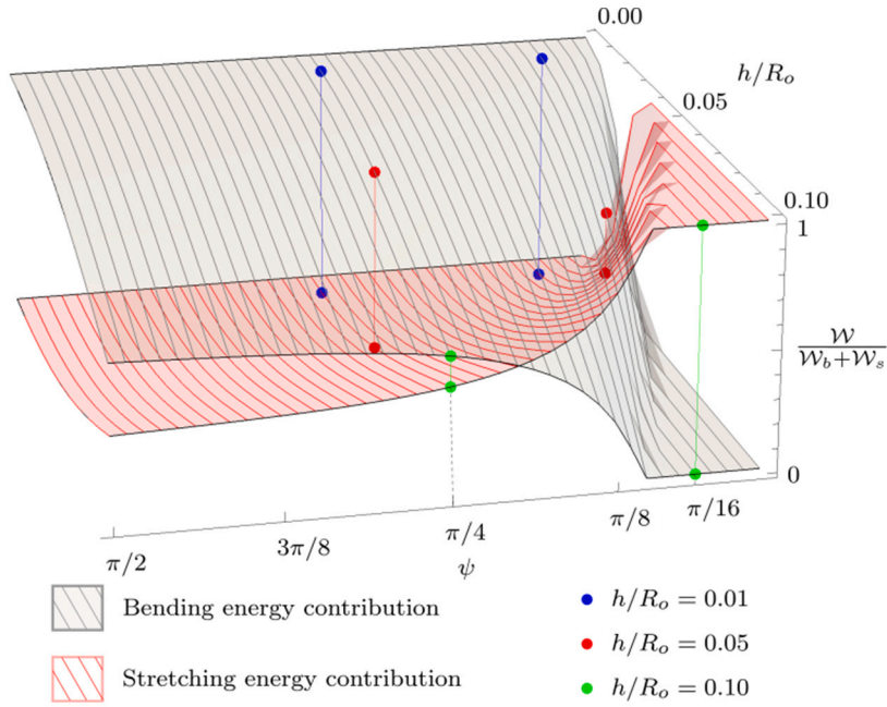
Fig. 9. Strain energy equipartition showing bending and stretching contributions as a function of the excess angle, \psi , and the plate's dimensionless thickness, h/R_o , for a creased e-cone ( m = 100 ) with a fixed lip rotation \eta = 0 . Vertical lines connect the corresponding stretching and bending contributions for equilibrium states with \psi = \pi/4, \pi/16 and h/R_o = 0.01, 0.05 , and 0.10 .
