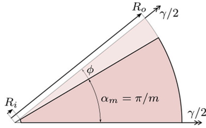
Fig. 3. Elastic panel deformation: a rotation on either edge equal to half the hinge rotation, i.e., \gamma/2 , and a stretch by changing its subtended angle from \alpha_m to \alpha_m + \phi .
