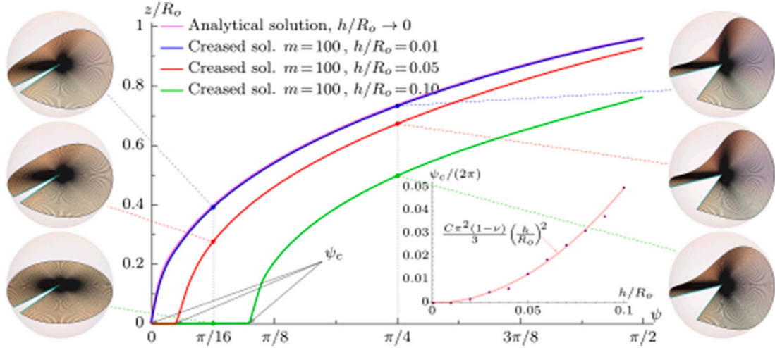
Fig. 8. Deflection of the antipodal point to the slit for increasing values of the excess angle, \psi , plotted for different thicknesses of the creased model with m = 100 . The near-threshold behaviour of finite thickness e-cones at the critical excess angle \psi_c can be clearly observed: unlike the isometric case where \psi_c = 0 , out-of-plane buckling is delayed for increasing thicknesses. In the inset, the critical excess angle, \psi_c , is plotted against the dimensionless thickness—data fitting identifies the quadratic scaling \psi_c \propto (h/R_o)^2 .
