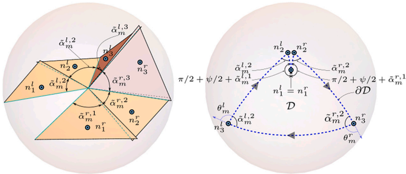
Fig. 11. Gauss map representation of a creased ( m = 3 ) e-cone with \psi = \pi/5 and \eta = 0 undergoing a combination of stretching and bending deformations. Unlike the Gauss map representation in Fig. 4, where the e-cone is only subject to bending, here stretching forces the panels to overlap at the creases, effectively reducing the subtended angles of the panels and with it the area of the spherical surface, D , enclosed by the path \partial D described by the surface normals.
