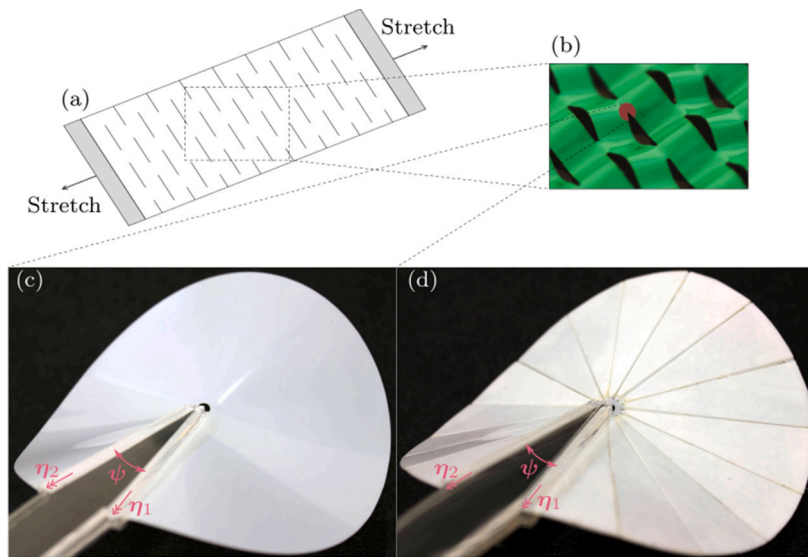
Fig. 1. Kirigami consists of making cuts in a flat sheet (a). The placement of such cuts endows the sheet with a higher capacity for stretching thanks to local out-of-plane buckling (b). Such buckling reduces to e-cone motifs locally forming around the tip of every cut, hence being the basic building bloc of kirigami. We show e-cones as a smoothly deformed surface (c) and a discretely deformed creased disk (d).
