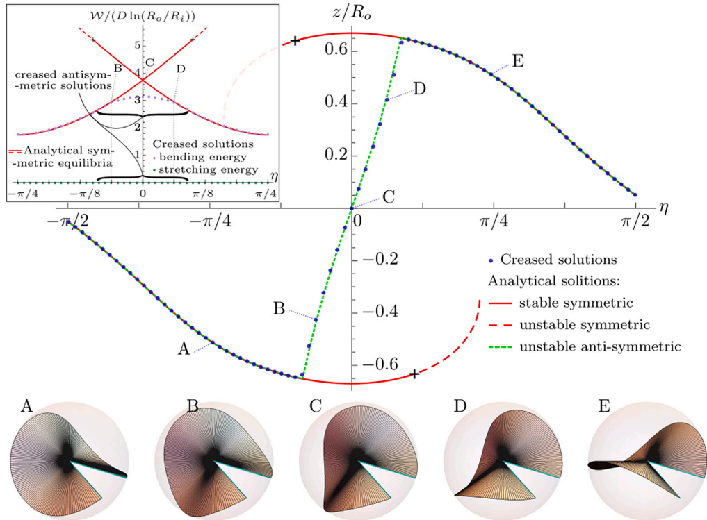
Fig. 7. Symmetric solution orbits and anti-symmetric connecting path for both the creased ( m = 100 ) and analytical (Sadik and Dias, 2021) solutions. The solutions are shown in the \{z/R_o, \eta\} phase space for h/R_o = 10^{-3} , with z being the deflection of the antipodal point to the slit. The inset shows the energy landscape for both the creased and analytical solutions. The + indicates the limit of stability for the symmetric solution.
