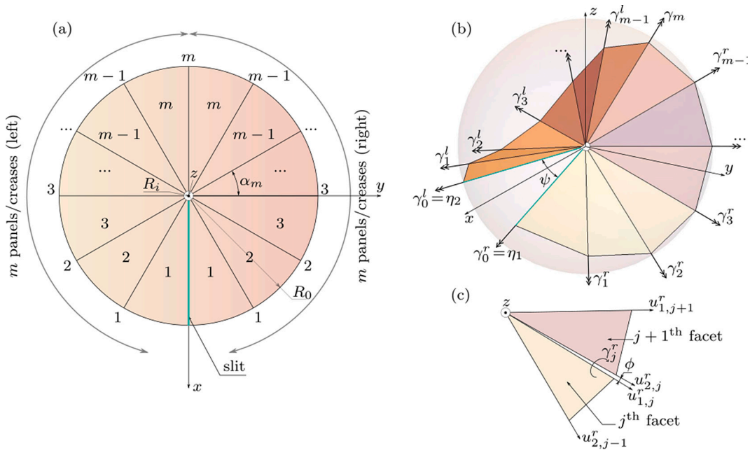
Fig. 2. Schematic diagrams for a creased annulus with inner radius R_i and outer radius R_o . (a) shows the creases layout, dividing each half-annulus into m facets of sector angle \alpha_m = \pi/m . The creases are numbered symmetrically, starting with the slit as 0 to m for the antipodal crease. (b) shows the annulus in the deformed configuration and indicates the rotation vectors between facets, \gamma_i , indicated as positive by a radially outward pointing vectors according to the right hand rule. Superscripts l and r indicate rotations on the left or right side of the annulus respectively. The two sides of the slit are opened to an angle of \psi and the imposed rotation angles at the slit lips labelled by \eta_1 = \gamma_0^r and \eta_2 = \gamma_0^l . (c) shows the labelling convention for the edge vectors of each facet. Edge vectors, u_{1,n} and u_{2,n} , are numbered in the clockwise direction on the right side and anti-clockwise on the left side, where n is the crease number—see (a). The superscript indicates which side (left - l, right - r) the facet is located on.
