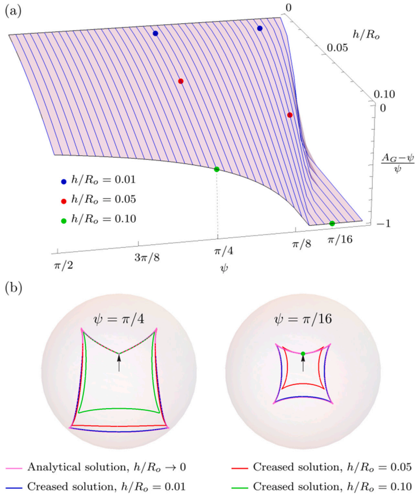
Fig. 10. (a) Gaussian charge deficit expressed as the relative difference between available Gaussian charge, A_G , and the excess angle, \psi , as a function of the dimensionless thickness, h/R_o , and the excess angle, \psi for a creased e-cone ( m = 100 ) with fixed lip rotation \eta = 0 . (b) Gauss map snapshots corresponding to points on (a) and Fig. 9 for selected values of \psi and increasing plate dimensionless thicknesses h/R_o . When the Gaussian charge is completely consumed by in-plane stretching, e.g., when \psi = \pi/16 and h/R_o = 0.1 , the Gauss map representation is reduced to a point.
