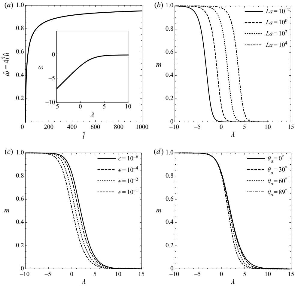
Figure 3. (a) Growth and saturation of the dimensionless bulk resistance, \hat{\omega} = 4\hat{l}\hat{u} , with the length of the imbibition front, \hat{l} , for parameter values La = 10 , \epsilon = 10^{-6} , \theta = 0^\circ and Bo = 0 . Inset: \omega = \ln \hat{\omega} vs \lambda = \ln \hat{l} . The cross-over between the linear growth of the front and the diffusive-like growth of Washburn's law is characterised by a transition of the exponent m = d\omega/d\lambda from m = 1 to m = 0 . (b–d) Variation of m with \lambda for different parameter combinations: (b) \epsilon = 1 , \theta_a = 0^\circ and Bo = 0 ; (c) La = 0 , \theta_a = 0^\circ and Bo = 0 ; (d) \epsilon = 10^{-6} , La = 0 and Bo = 0 .
