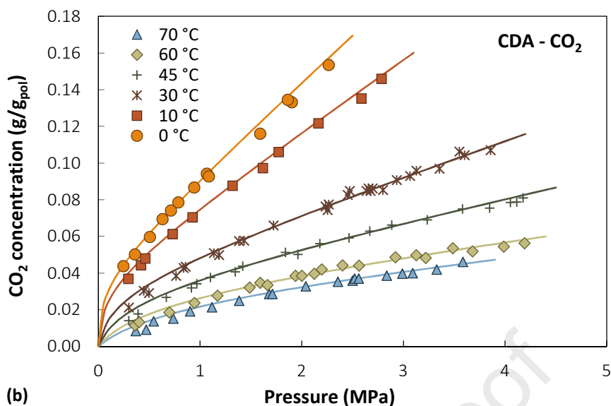
Figure 6. Experimental sorption isotherms of (a) CH 4 (ref. [84]) and (b) CO 2 (ref. [83]) in cellulose diacetate at different temperatures, together with NELF model calculations.
