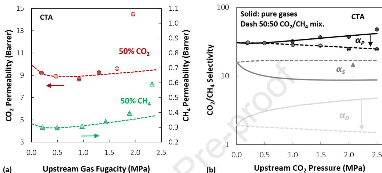
Figure 8. (a) Permeability of CO 2 (red) and CH 4 (green) in CTA at 35 °C. Experimental data from ref. [81]: symbols represent mixed gas data at equimolar composition. Dashed lines represent ST model predictions. (b) Perm-selectivity (black), solubility- (gray) and diffusivity-selectivity (light gray) of CO 2 /CH 4 at ideal conditions (solid lines) and for an equimolar mixture (dashed) predicted by the ST model. Symbols are experimental perm-selectivity from ref. [81].
