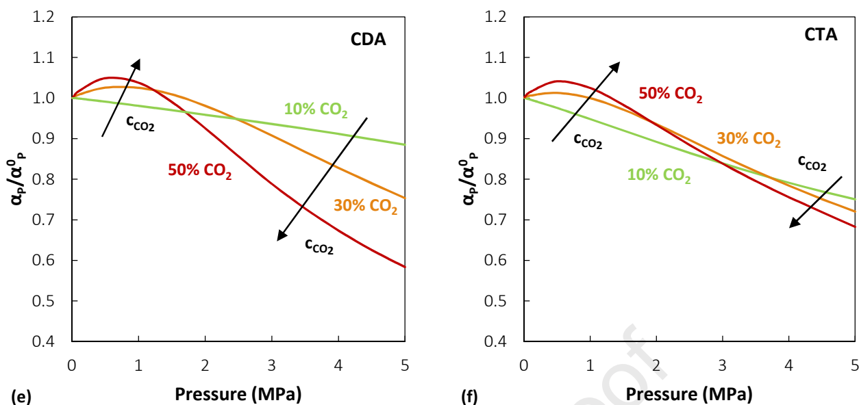
Figure 14. Ratio of ideal and multicomponent \text{CO}_2/\text{CH}_4 solubility-selectivity, diffusivity-selectivity and permselectivity in CDA and CTA calculated with the NELF and ST models at 35 °C and at different mixture compositions: 10/90 mol% in green, 30/70 mol% in orange, 50/50 mol% in red. The arrows point in the direction of increasing \text{CO}_2 content in the gas phase. Ratios performed taking values of pure and mixed gas properties at the same gas fugacity value.
