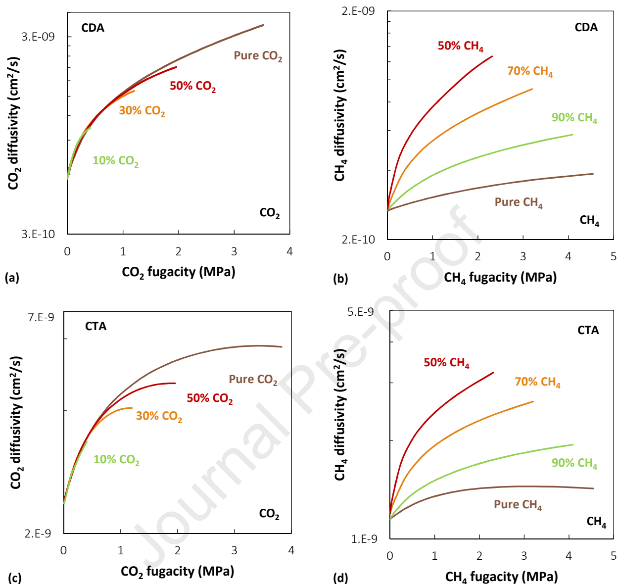
Figure 11. Mixed gas diffusion coefficients of 10/90 (green), 30/70 (orange) and 50/50 (red) mol% CO 2 /CH 4 mixtures in CTA and CDA at 35 °C calculated from the solution-diffusion relation. The brown lines represent pure gas diffusion coefficients.
