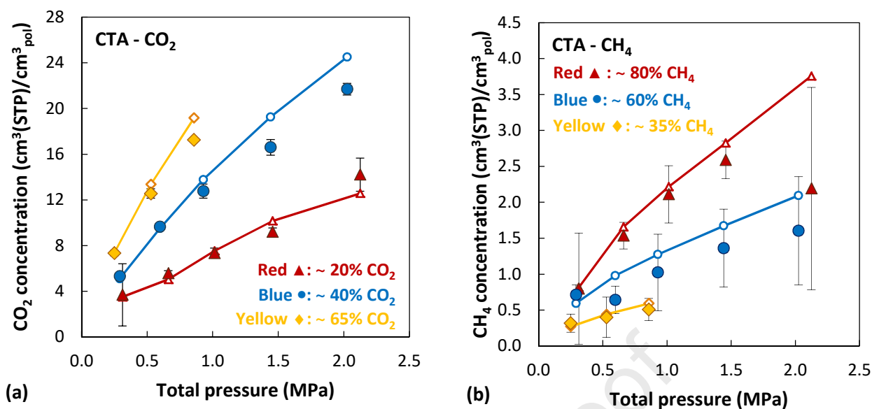
Figure 7. Mixed gas sorption of \text{CO}_2 and \text{CH}_4 in CTA. Filled symbols: experimental data from ref. [5]. Empty symbols with solid lines: NELF model predictions. Colors and symbols represent data at similar mixture composition to facilitate the visualization, however each point was calculated at its corresponding equilibrium composition, reported in the original reference and also in Table S4 for convenience.
