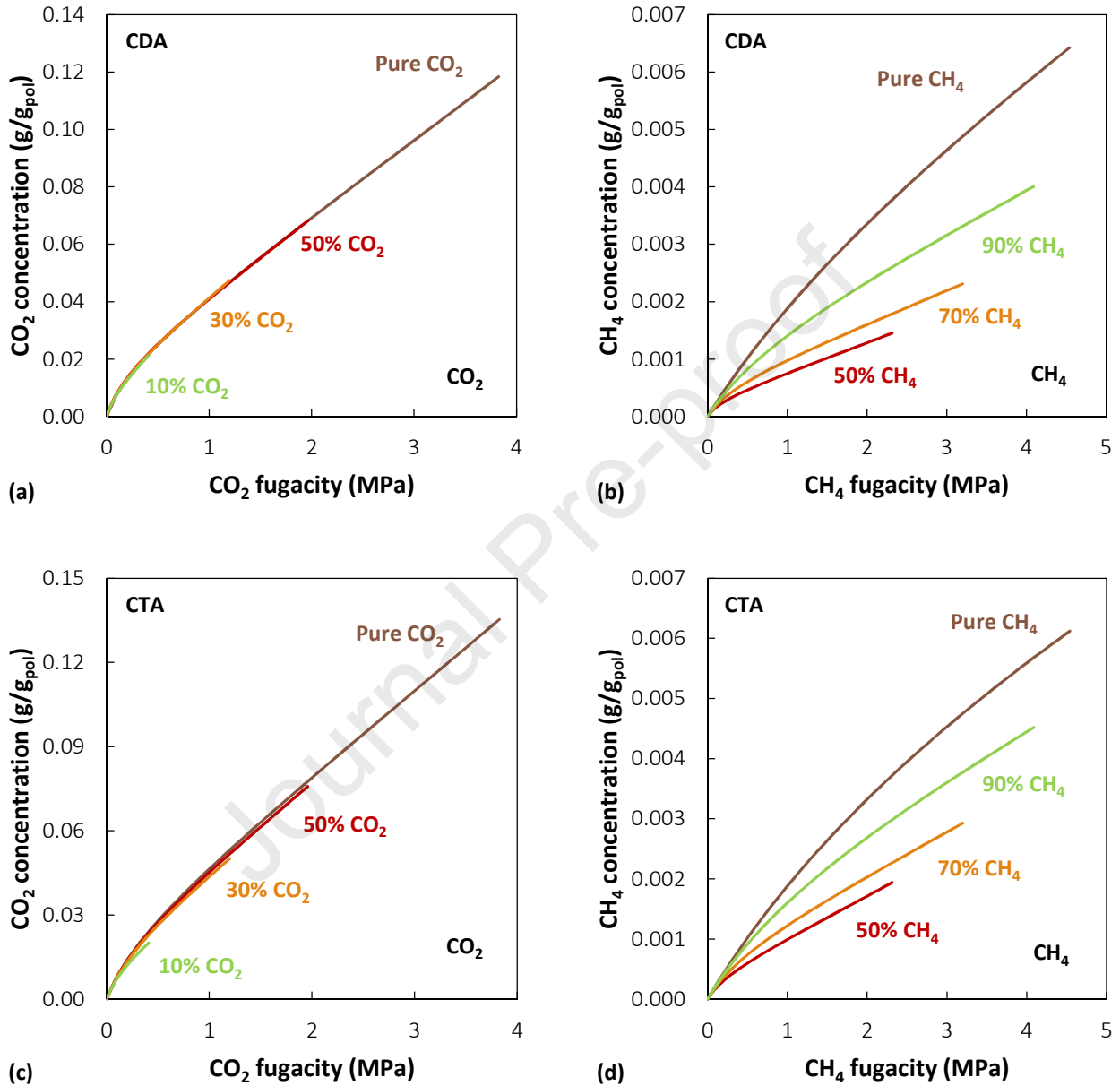
Figure 10. Mixed gas sorption of 10/90 (green), 30/70 (orange) and 50/50 (red) mol% CO 2 /CH 4 mixtures in CTA and CDA at 35 °C calculated with the NELF model. The brown lines represent pure gas sorption.
