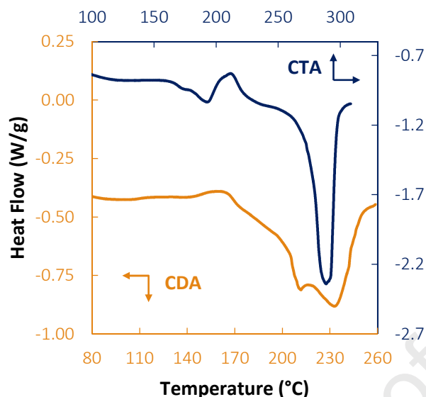
Figure 1. Representative DSC thermograms for CDA (orange, read on lower and left axis) and CTA (blue, read on upper and right axis), magnified in the regions of recorded transitions and recorded during the first heating scan. Exothermic transitions are displayed by positive peaks in DSC curves.
