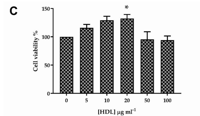
Figure 1. The effects of treatment (24 h) with HDL (0–100 \mu\text{g mL}^{-1} ) on the conversion of MTT to formazan by HKn, HDFn and HDFa are shown in (A–C), respectively; data in each figure are the mean \pm SEM of three independent experiments, each performed using six replicates. The data were analysed using one-way ANOVA and Dunnett’s post-hoc test; * p < 0.05 .
