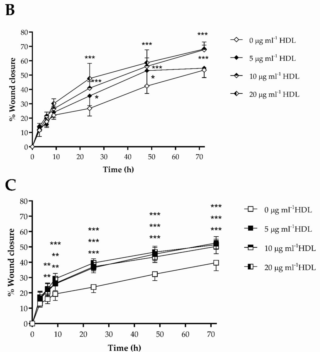
Figure 3. ‘Scrape’ wound healing, in the presence or absence of HDL (5–20 µg mL -1 ; 0–72 h), compared with the control (serum-free media) condition, by HKn, HDFn and HDFa, are shown in (A–C), respectively. Data are the mean ± SEM of three independent experiments (each performed using triplicate wells). The data were analysed using two-way ANOVA and Tukey post-hoc test; * p < 0.05 ; ** p < 0.01 ; *** p < 0.001 . In (C), after 6 h, significance ( p < 0.01 ) from control is noted after treatment with HDL (5 µg mL -1 and 20 µg mL -1 ); at 9 h, significance is noted for 5 µg mL -1 ( p < 0.01 ), 10 µg mL -1 ( p < 0.001 ) and 20 µg mL -1 ( p < 0.001 ); for time points thereafter, significance ( p < 0.001 ) from control is noted for all three concentrations tested.
