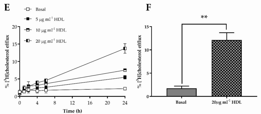
Figure 2. The dose and time dependencies of [ 3 H]cholesterol efflux to HDL from HKn, HDFn and HDFa are shown in (A,C,E), respectively: data in each of these figures are from a single experiment and values shown are the mean ± S.D of triplicate wells. (B,D,F) show [ 3 H]cholesterol efflux measured in three independent experiments (each performed using triplicate wells), from HKn, HDFn and HDFa, respectively; values are mean ± SEM. The data were analysed using a Student’s t -test (paired, two way); ** p < 0.01. The data from experiments in (B,D,F) were compared using a one-way ANOVA and Tukey post-hoc test.
