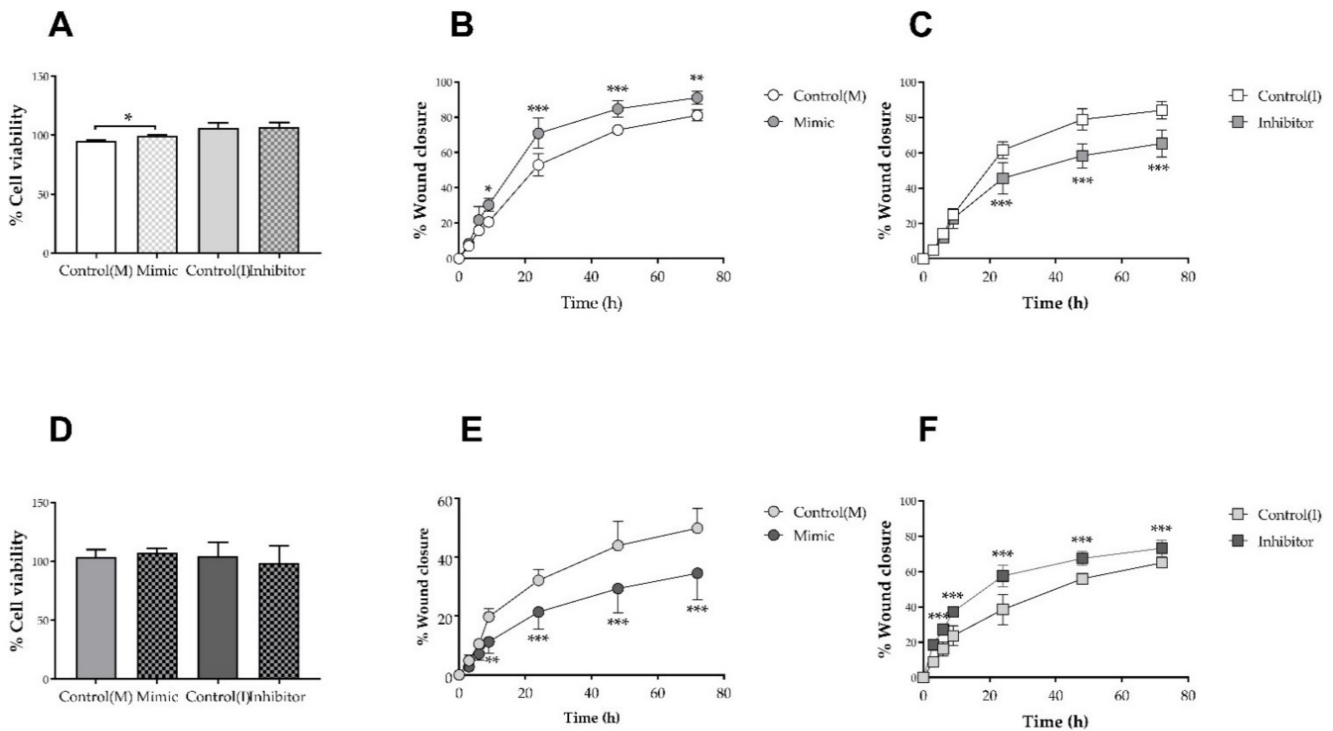
Figure 6. The effects of treatment (24 h) with hsa-mir-6727-6p mimic (10 nM; 24 h) and inhibitor (50 nM; 24 h) on the conversion of MTT to formazan by HDFn and HDFa, compared with the relevant SiRNA scrambled control are shown in (A,D), respectively; data in each figure are the mean ± SEM of three independent experiments, each performed using six replicates. The data were analysed using a Student’s paired t -test; * p < 0.05. ‘Scrape’ wound healing (0–72 h) in the presence of the same concentrations of mimic (B,E) and inhibitor (C,F) compared with relevant SiRNA scrambled controls, are shown in HDFn (B,C) and HDFa (D,F). Data are the mean ± SD of four independent experiments, each performed using duplicate wells; SD was utilised as error bars were too small to indicate the variance of the data using SEM. The data were analysed using two-way ANOVA and Tukey post-hoc test; * p < 0.05, ** p < 0.01; *** p < 0.001.
