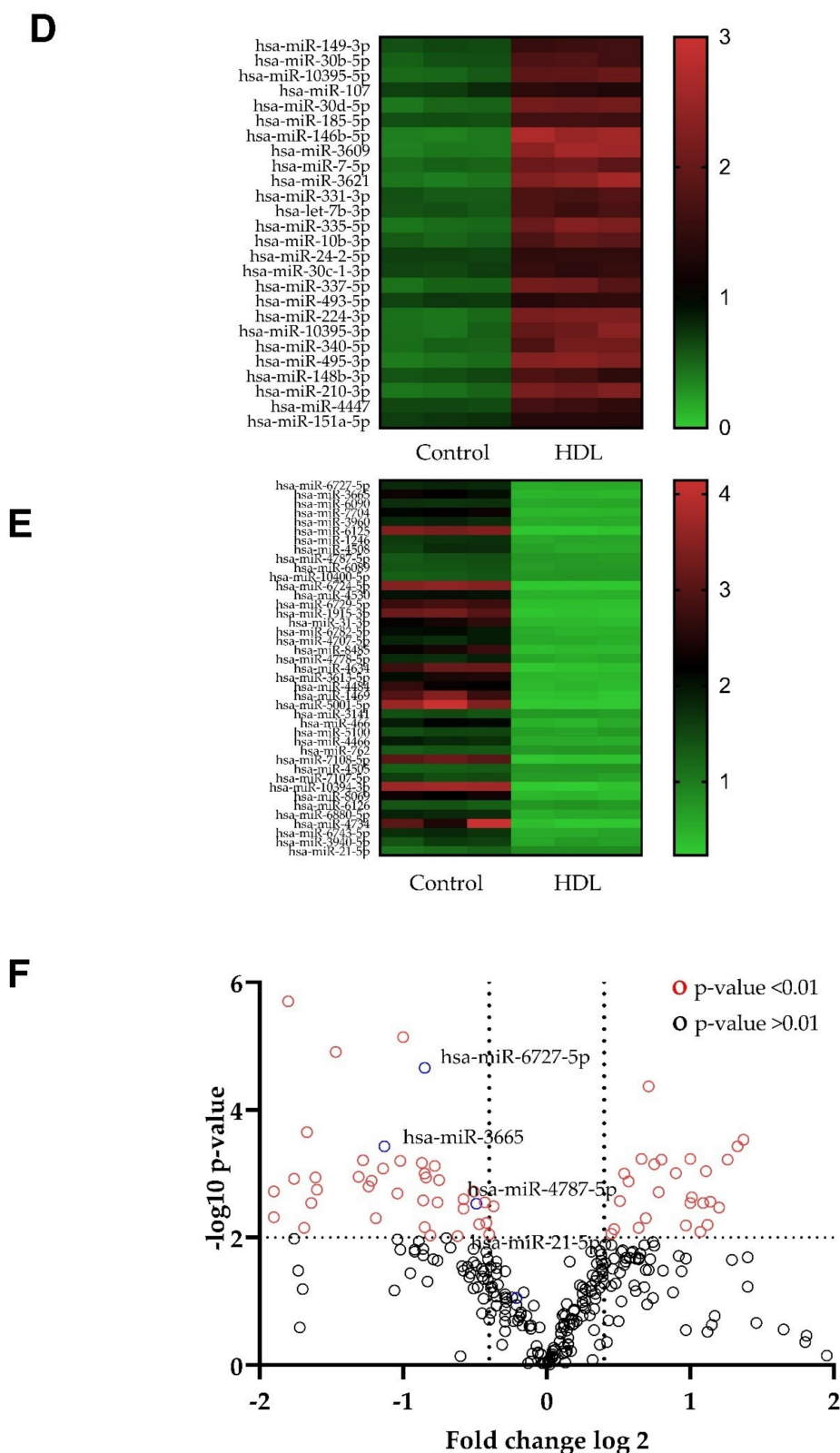
Figure 4. Heatmaps and volcano plots depicting miRNAs regulated following 24 h treatment with 20 \mu\text{g ml}^{-1} HDL, compared with the relevant control, in neonatal human dermal fibroblasts (A–C) and adult human dermal fibroblasts (D–F). Data are presented from one sample per group, each with an independent microchip array containing three technical replicates per sequence on each microchip. All miRNAs presented show differences p < 0.05 (Student’s t -test) compared to the basal control, and are ranked in order of statistical significance.
