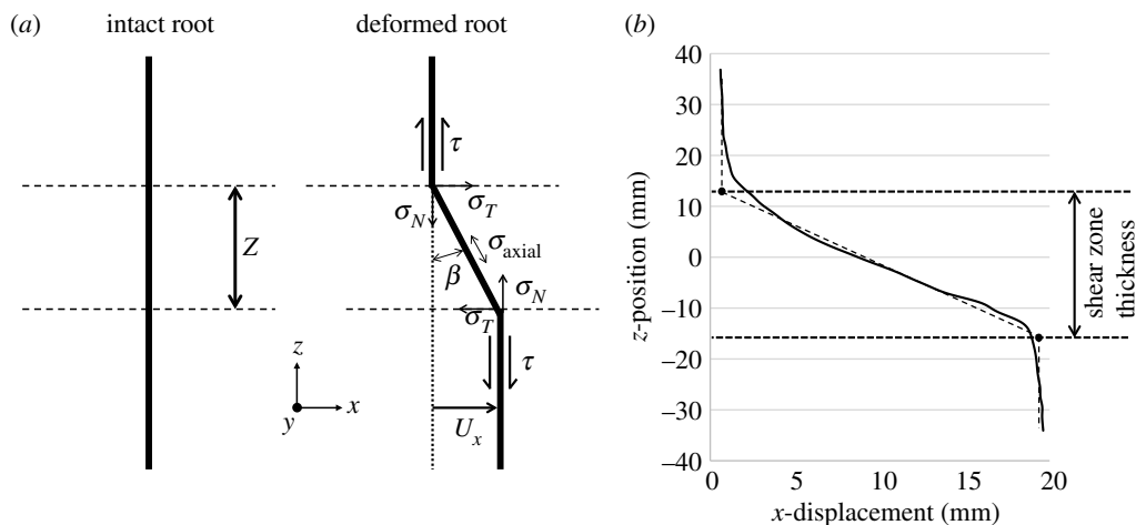
Figure 2. (a) Schematic illustrating the development of root stresses during direct shear [22]. (b) Example of tri-linear fit (dotted line) used to determine local shear zone thickness from z -position versus x -displacement (solid line) DVC data. The shear zone thickness was calculated at every (x, y) position on the shear plane, for each displacement step in the test.
