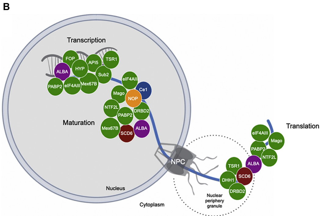
FIG. 12. Schematic representation of T. cruzi mRNA export machinery. A , using a cohort of six affinity handles, we identified a large interactome that illustrates multiple interactions as well as the presence of conserved and divergent proteins. Furthermore, these data validate the absence of many components that have failed to be identified in silico , including proteins of the TREX and TREX2 complexes. Cohorts are arranged as identified in the pullouts and colored by predicted function using the scheme as in Tables 1 and 2 . Large boxes represent a single interactome, with the affinity handle indicated. Dotted lines between entries indicate a detected interaction. Many potential interactions and the TcMex67 isolation have been omitted for clarity. Conserved proteins include TcSub2, TcelF4AIII and multiple RNA binding proteins and EJC components. kinetoplastid-specific proteins include TcAPI5, TcFOP and TcNTF2L, and TcFOP and TcAPI5 interact directly with TcSub2. Core components of the EJC are directly associated with the mRNA machinery. TcNTF2L seems to be a shuttling protein that interacts with TcelF4AIII and the export receptor TcMex67. Connectivity data are also available as a cytoscape file for readers who wish to explore further. B , model for interactome and interactions with the NPC and export systems. Conserved proteins, such as TcSub2, TcelF4AIII, RNA binding proteins, components of the EJC, and kinetoplastid-specific proteins, such as TcAPI5, TcFOP, and TcNTF2L are shown. The nuclear proteins TcFOP and TcAPI5 interact directly with TcSub2. Core components of EJC are directly associated to mRNA machinery. TcNTF2L seems to be a shuttling protein that interacts with TcelF4AIII and the export receptor TcMex67.
