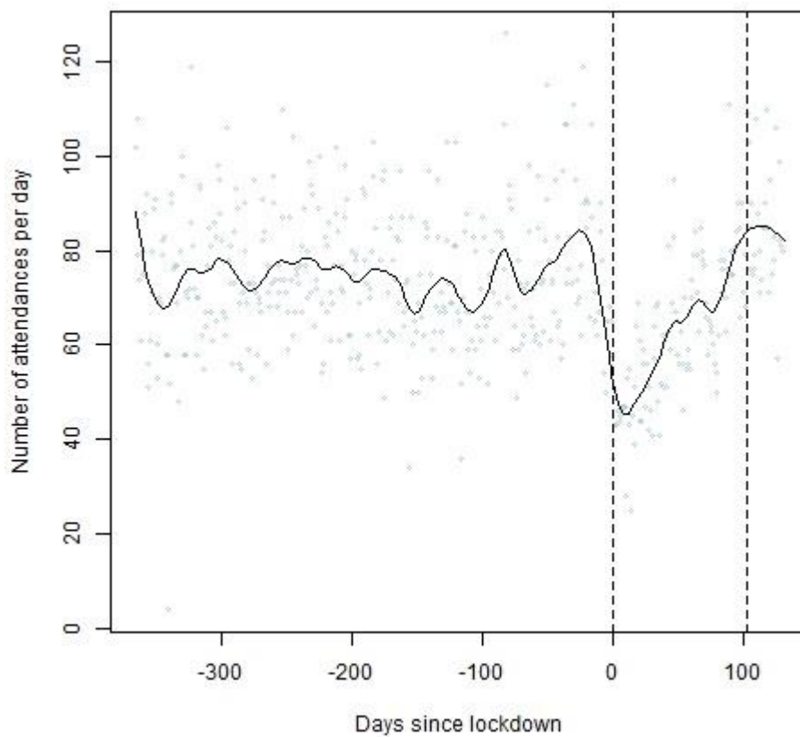
Figure 1: Smoothed B-spline of alcohol/substance use attendances per day
