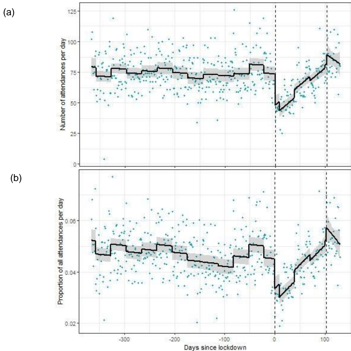
Figure 2: Interrupted time series 1 plot of alcohol/drug use for (a) total count and (b) proportion compared to all attendances
