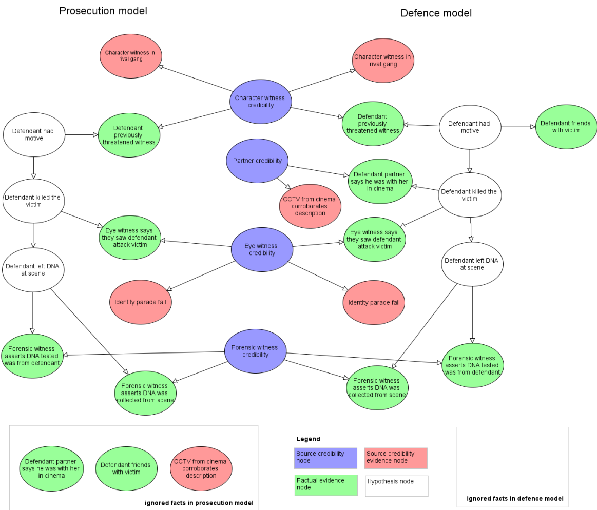
Figure 4 Revised prosecution, m_P , and defence models, m_D
