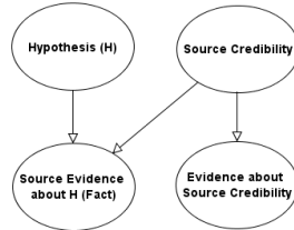
Figure 3 Model showing evidence accuracy idiom
