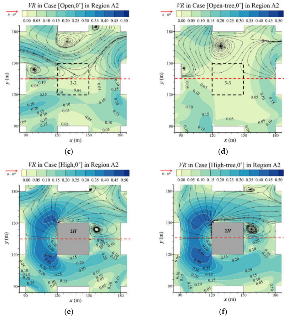
Figure 3. Streamline and velocity ratio (VR) at z = 2\text{m} in Region A2 in (a) Case [Base, 0^\circ ], (b) Case [Base-tree, 0^\circ ], (c) Case [Open, 0^\circ ], (d) Case [Open-tree, 0^\circ ], (e) Case [High, 0^\circ ] and (f) Case [High-tree, 0^\circ ].
