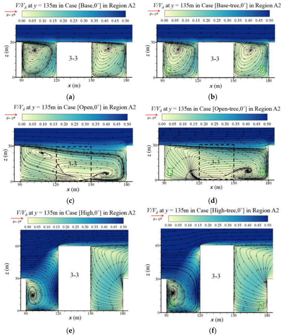
Figure 4. Normalised velocity ( V/V_\delta , V_\delta = 4.34\text{ m/s} ) at vertical plane ( y = 135\text{m} ) in Region A2 in (a) Case [Base, 0^\circ ], (b) Case [Base-tree, 0^\circ ], (c) Case [Open, 0^\circ ], (d) Case [Open-tree, 0^\circ ], (e) Case [High, 0^\circ ] and (f) Case [High-tree, 0^\circ ].
