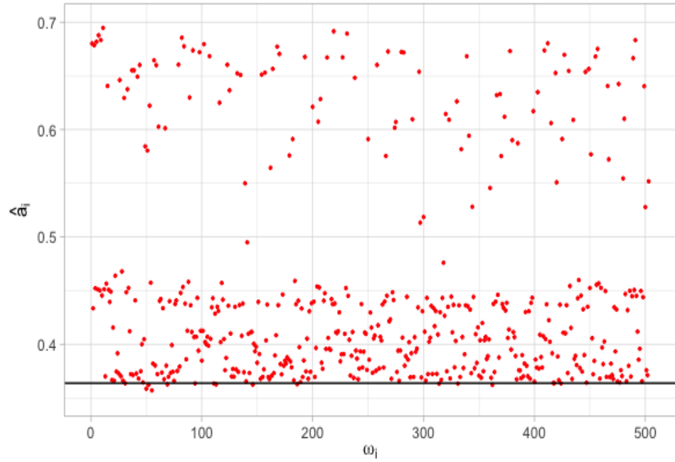
Figure 3.4: Posterior mean of the score parameters represented by the red dots and the optimal threshold as the horizontal black line.
