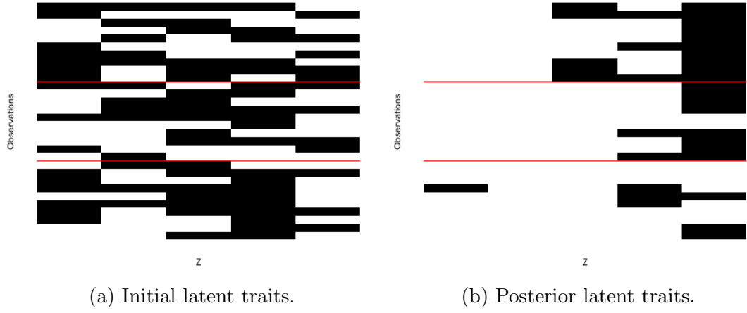
Figure 4.8: Evolution of the dynamics of the binary matrix of latent traits Z .
