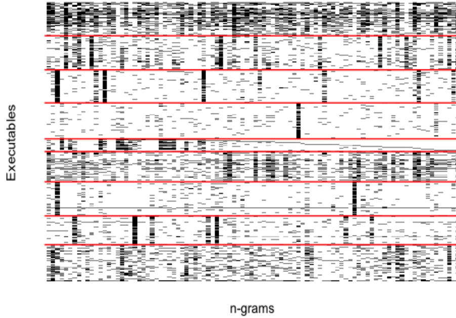
Figure 3.8: Graphical representation of the data set comprised of 590 malware (rows) of nine families separated with the solid horizontal lines and the 96 features selected through the generalised beta-CoRM. The dots represent the features that appear in each executable.
