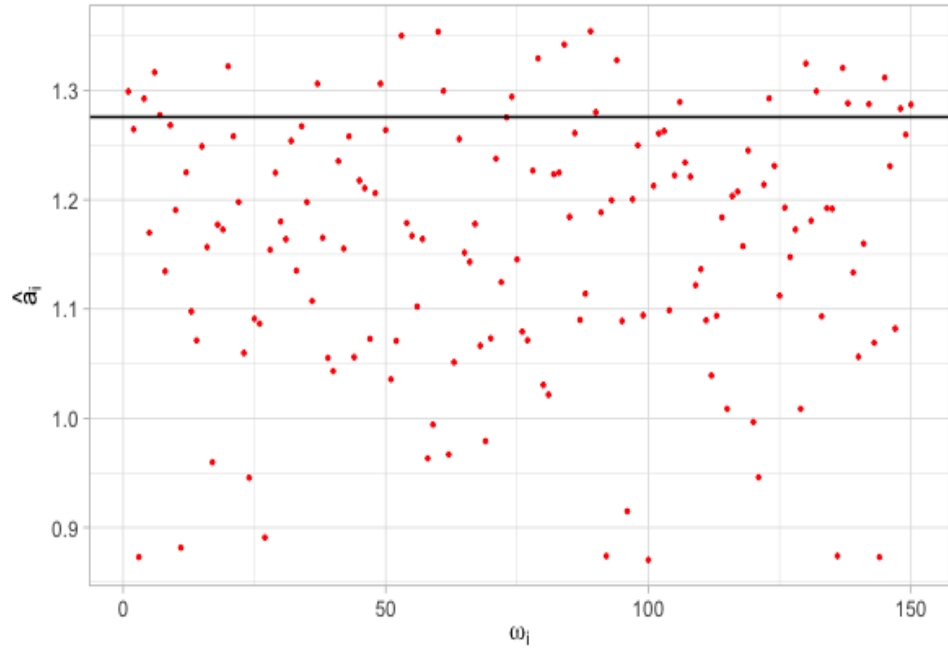
Figure 3.2: Posterior estimates of the respective score parameter a_i for each feature, along with the optimal threshold represented by the black horizontal line.
