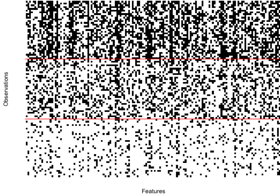
Figure 2.2: Synthetic binary matrix comprised of 150 features (columns) and 100 observations (rows) divided into three well-defined groups separated by the horizontal red lines. The dots representing the features present for each observation.
