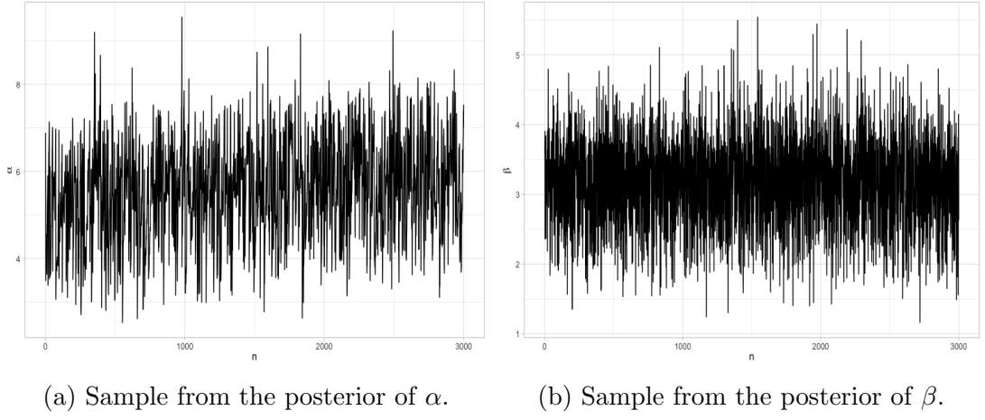
Figure 3.1: Posterior samples of the hyperparameters \alpha and \beta corresponding to the distribution of the score parameters.
