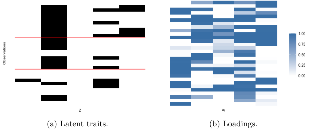
Figure 4.1: The latent traits and the loadings generated by the beta-CoRM BMF generative process with parameters (\gamma, c, R, a, \alpha, \beta) = (2, 1, 5, 1, .1, .1) .
