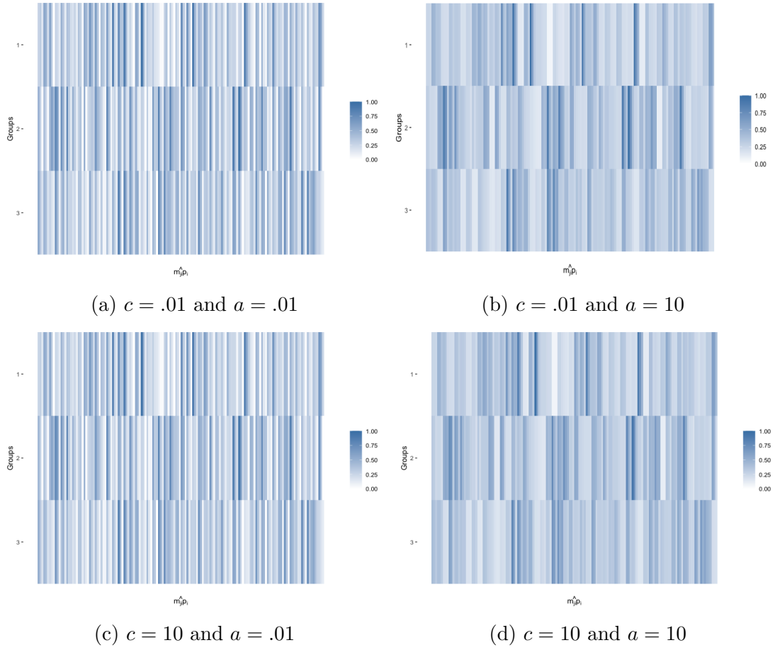
Figure 2.6: Comparison of the posterior predictive probabilities between the beta-CoRM with a small a (left) and with a large a (right) for the data illustrated in Figure 2.2.
