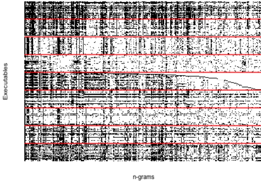
Figure 4.9: Graphical representation of the malware data composed of 270 observations and 335 features divided evenly into nine families separated by the red lines.
