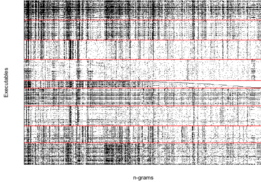
Figure 2.7: Graphical representation of the data set comprised of 590 malware (rows) of 9 families separated with the solid horizontal lines and 826 4-grams (columns). The dots represent the features that appear in each executable.
