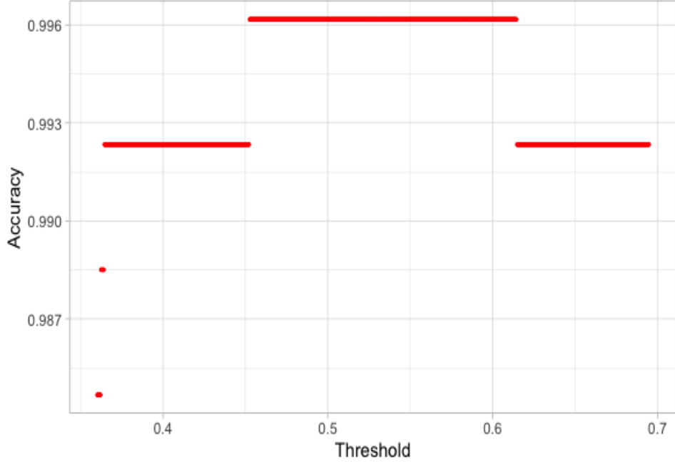
Figure 3.5: Accuracy for different thresholds.
