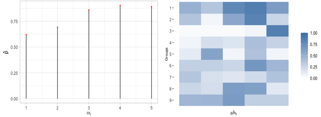
(a) Posterior estimates of the beta process' jumps. (b) Posterior estimates of the groups' probabilities.
