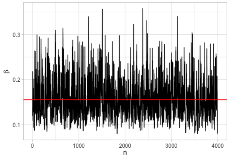
Figure 4.7: Posterior samples of \beta . The horizontal red line represents the mean.
