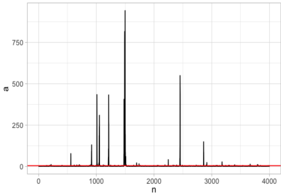
Figure 4.5: Posterior samples of a . The horizontal red line represents the mean.
