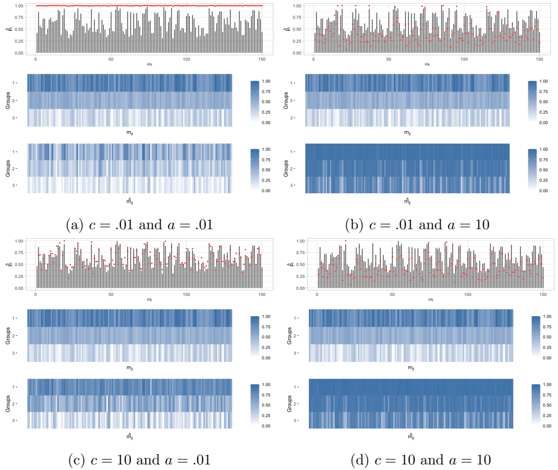
Figure 2.4: Posterior inference results for the beta-CoRM model with different choices of c and a for the data illustrated in Figure 2.2. For each subplot: Upper graph: real probabilities (spikes) and posterior estimates (red dots). Middle graph: real scores. Bottom graph: posterior estimates of the scores.
