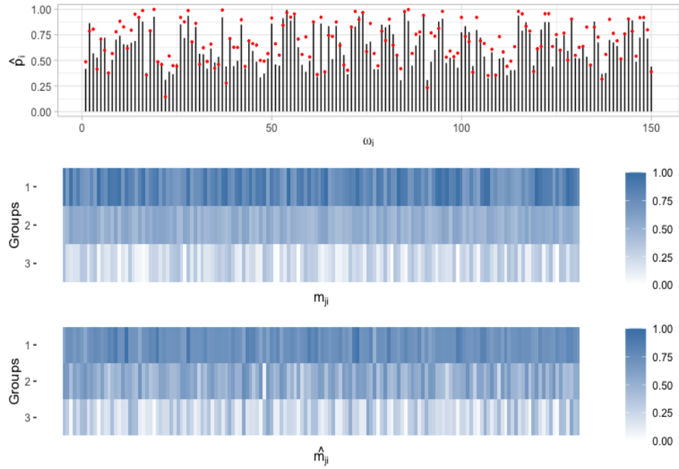
Figure 2.3: Posterior inference results of the beta-CoRM models for the data illustrated in Figure 2.2. Upper graph: real probabilities (spikes) and posterior estimates (red dots). Middle graph: real scores. Bottom graph: posterior estimates of the scores.
