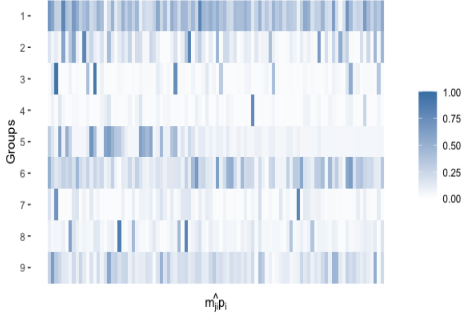
Figure 3.10: Posterior probability of each of the 96 features appearing in each of the 9 families of the malware classification data set.
