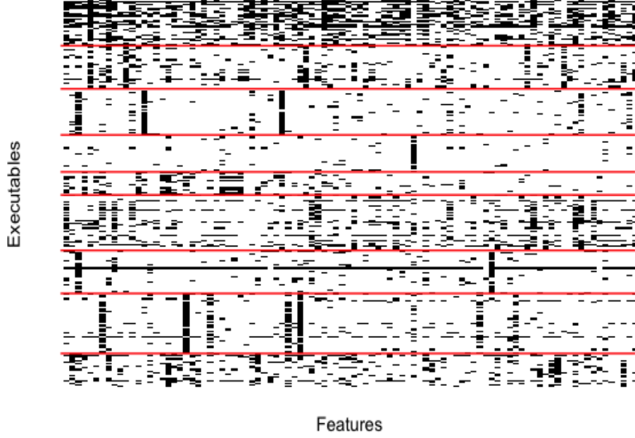
Figure 3.9: Graphical representation of the test set comprised of 252 malware (rows) of nine families separated with the solid horizontal lines and the 96 features selected through the generalised beta-CoRM. The dots represent the features that appear in each executable.
