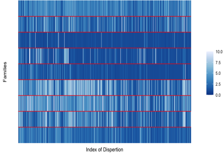
Figure 5.3: Index of dispersion for each feature across families.
