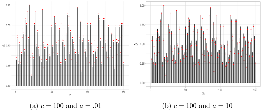
Figure 2.5: Comparison between the posterior estimates of the jumps of the directing beta process (red dots) and the q_i 's (spikes) for a large value of c and for a small and a large value of a .
