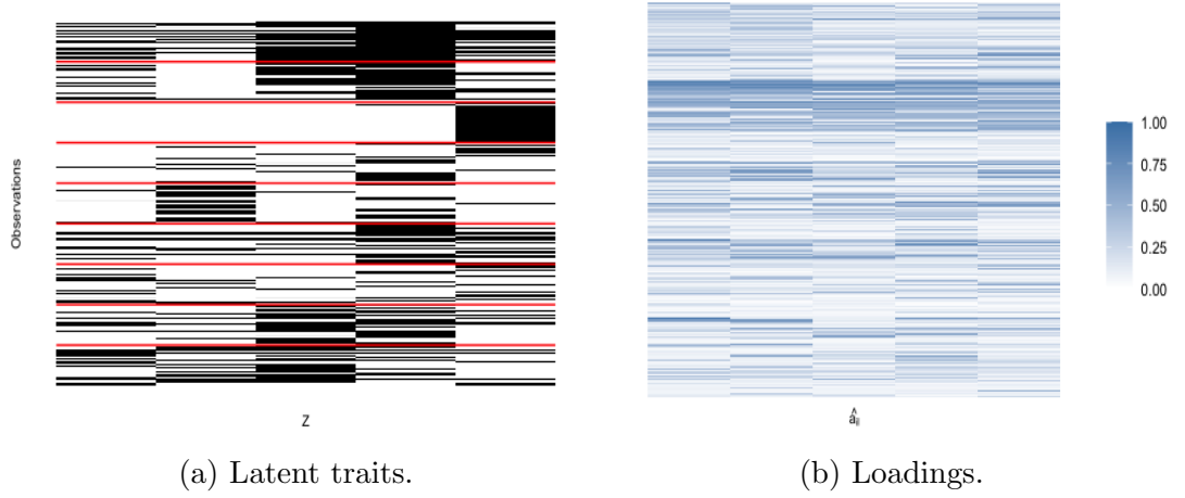
Figure 4.10: The inferred latent traits and loadings for the malware data set described in Figure 4.9.
