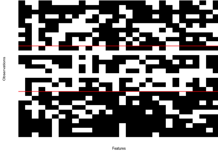
Figure 4.2: Synthetic data generated by the beta-CoRM BMF generative process with parameters (\gamma, c, R, a, \alpha, \beta) = (2, 1, 5, 1, .1, .1) .
