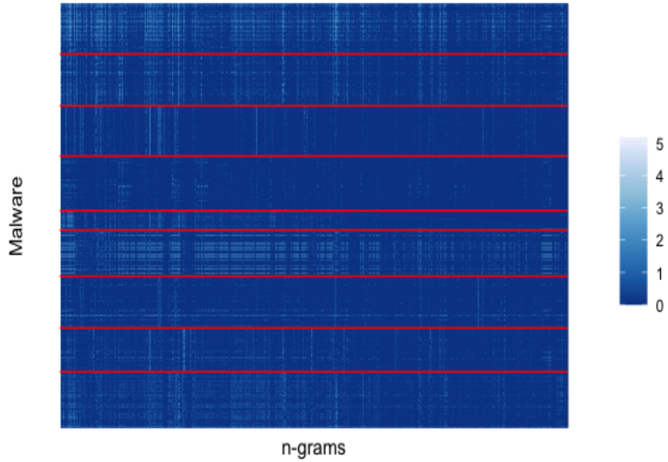
Figure 5.1: Intensity of each feature calculated as \log_{10}(X_{ij} + 1) across each of the nine families of malware separated by the red lines.
