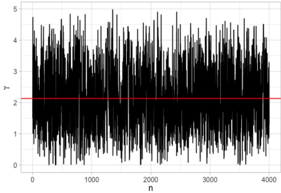
Figure 4.4: Posterior samples of \gamma . The horizontal red line represents the mean.
