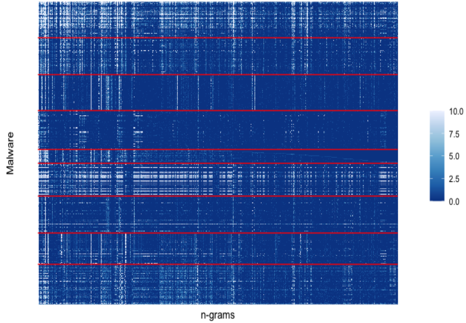
Figure 5.2: Matrix of truncated counts (at 10) across each of the nine families of malware separated by the red lines.
