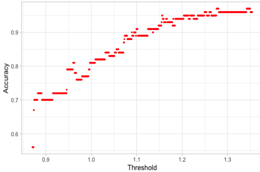
Figure 3.3: Accuracy performance for different threshold levels.
