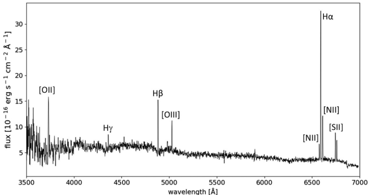
Figure 1. Obtained INT spectrum of Type Ib SN2012au environment as an example for the extracted 1D environment spectra. The figure shows the most prominent emission lines of which H\alpha , [NII] \lambda 6583 , H\beta , and [OIII] \lambda 5007 have been used for the metallicity estimation.
