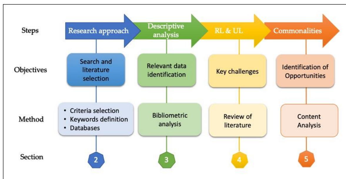
Figure 1. Methodological approach.
