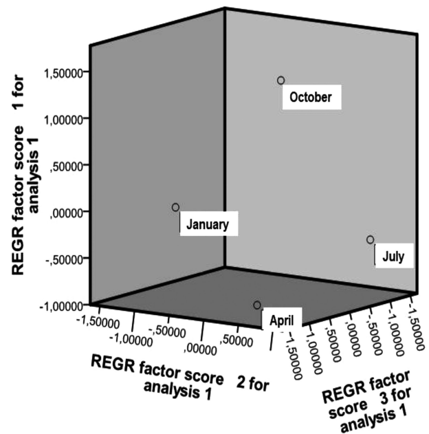
Figure 4 | 3D factorial analysis plot.
