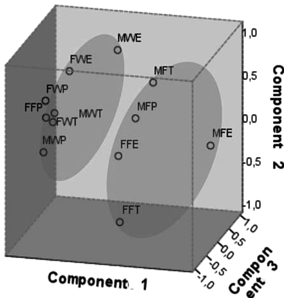
Q2 Figure 3 | 3D scatter plot of principal components: Left cluster : MWE = male (wild) estradiol, FWE = female (wild) estradiol, FWP = female (wild) progesterone, MWT = male (wild) testosterone, FWT = female (wild) testosterone, MWP = male (wild) progesterone. Right cluster : MFT = male (farmed) testosterone, MFP = male (farmed) progesterone, FFE = female (farmed) estradiol, MFE = male (farmed) estradiol, FFT = female (farmed) testosterone. Unexpected location : FFP = female (farmed) progesterone.
