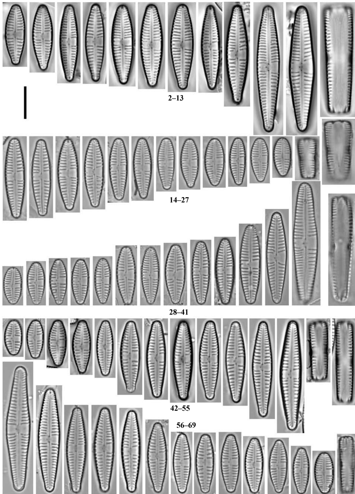
Figs 2–69. Light micrographs of Gomphonema rosenstockianum : (2–13) type material, La Gomera, Canary Islands, Spain; (14–27) Arão Stream, Pereira, South of Portugal; (28–41) Algre Stream, Tôr, South of Portugal; (42–55) Son Brull Stream, Pollença, Mallorca, Spain; (56–69) Puigpunyent Stream, Puigpunyent, Mallorca, Spain. Scale bar 10 \mu m.
