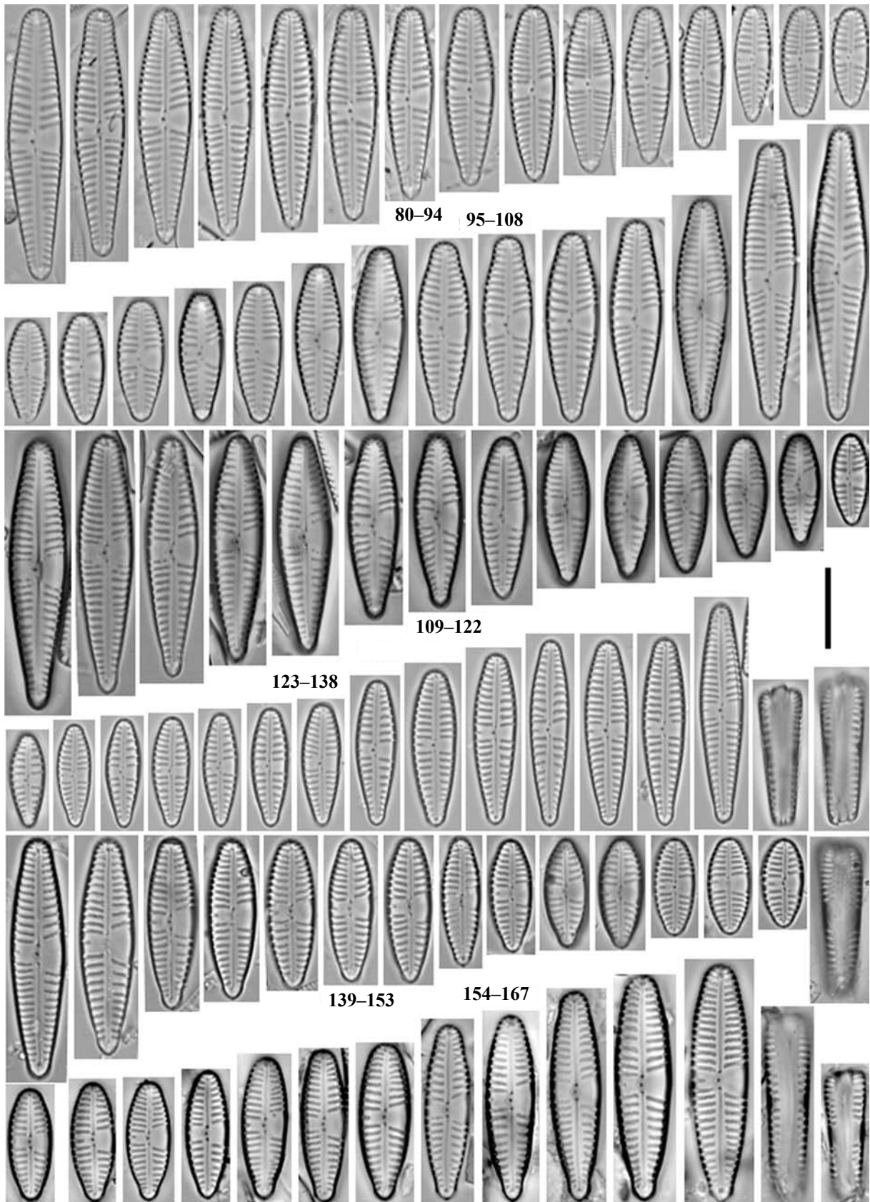
Figs 80–167. Light micrographs of Gomphonema tergestinum : (80–94) Cant Stream, Biancot, Cuneo, Italy; (95–108) Germanasca Stream, Ghigo di Prali, Torino, Italy; (109–122) Payant Stream, Bobbio Pellice, Torino, Italy; (123–138) Drôme River, Charens, Rhone Alps, France; (139–153) Danube River, Karlova Ves, Slovakia; (154–167) Lomnica River, Juskova Vola, Slovakia. Scale bar 10 \mu m.
