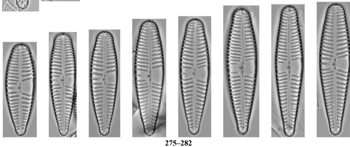
Figs 253–265. Light micrographs of Gomphonema angustius from Arba de Biel River, Luna, Zaragoza, Spain.
