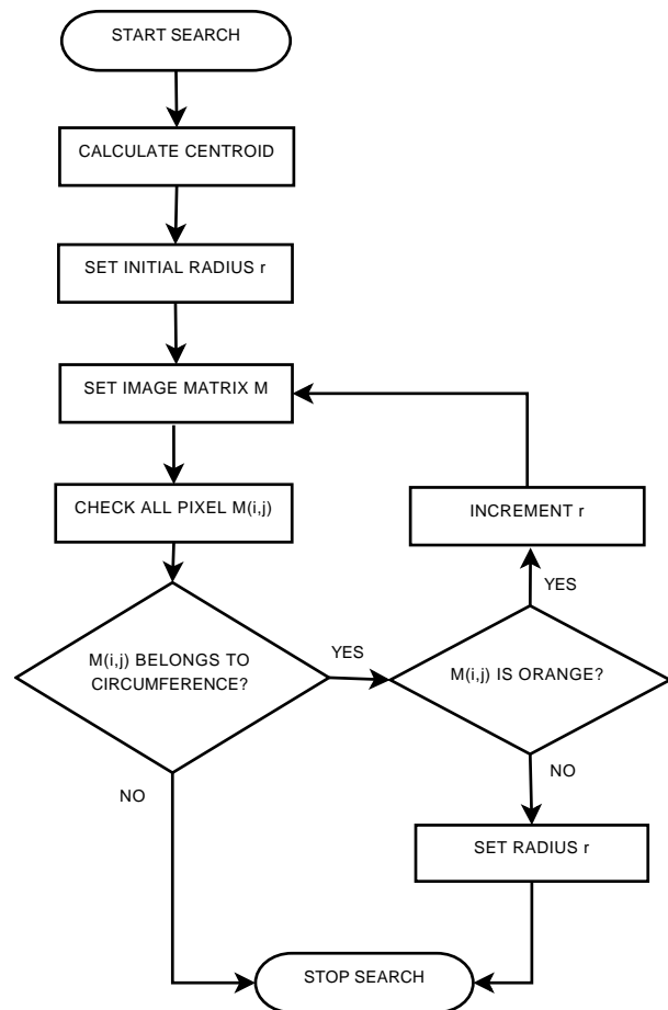
Fig. 5. Step one: circle's radius calculation
