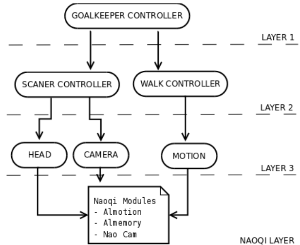
Fig. 2. Hierarchy of controllers implementing the goalie behavior
