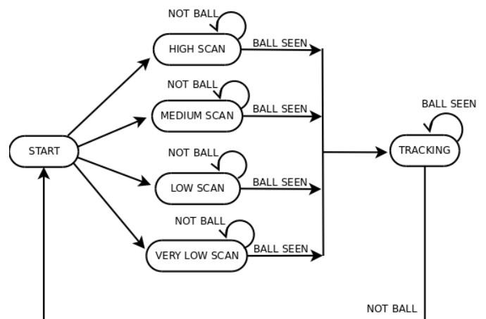
Fig. 4. Scanner state automata
