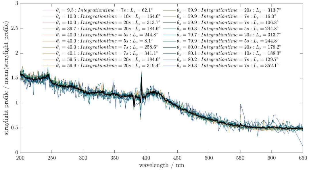
Fig. 5. The inflight straylight profile as a function of wavelength at pixel position ( p_{m,t_0} - p_{s,t_0} ) in the NLR for different, solar zenith angles, location, integration times and time of year. Each straylight profile has been normalised to the mean of itself across all wavelengths to emphasise that the straylight is independent of the incident flux, integration time and has been stable over the course of the UVIS science mission. The mean straylight structure as a function wavelength is shown by the black line.
