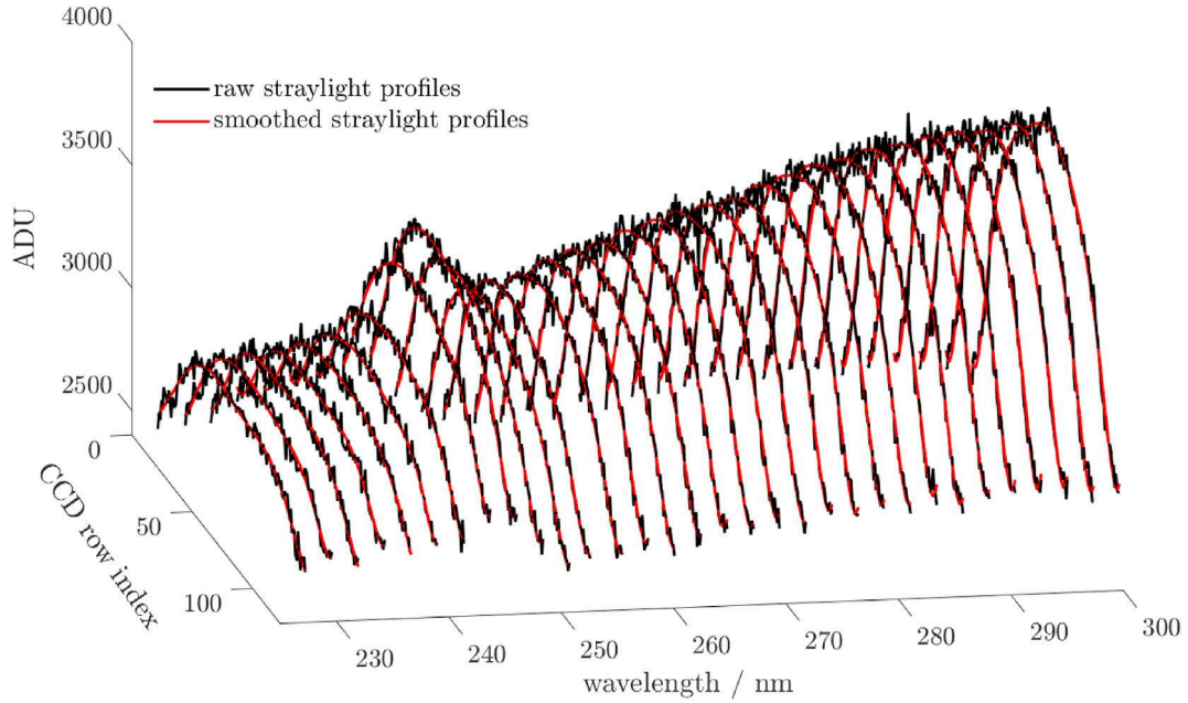
Fig. 3. The raw and fitted straylight profiles for wavelengths between 225 nm and 300 nm are shown in 2.3 nm steps (every 5 CCD columns) for clarity.
