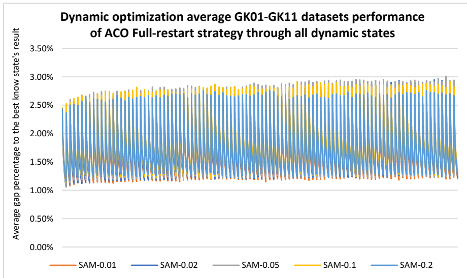
490 Fig. 10. Dynamic optimization performance of ACO Full-restart strategy for all SAM levels. Each line shows the average gap convergence of GK01-GK11 dynamic datasets group run 10 times each, totalling 110 runs.
