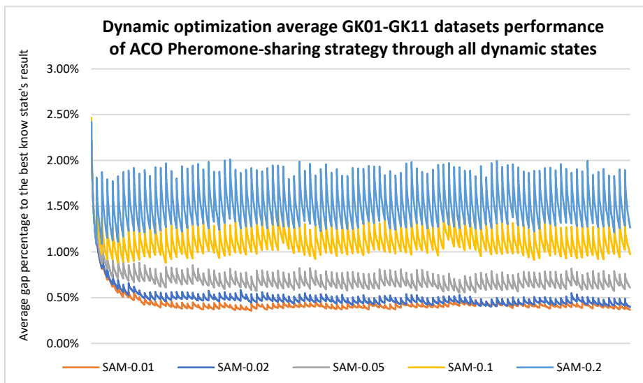
495 Fig. 11. Dynamic optimization performance of ACO Pheromone-sharing strategy for all SAM levels. Each line shows the average gap convergence of GK01-GK11 dynamic datasets group run 10 times each, totalling 110 runs.
