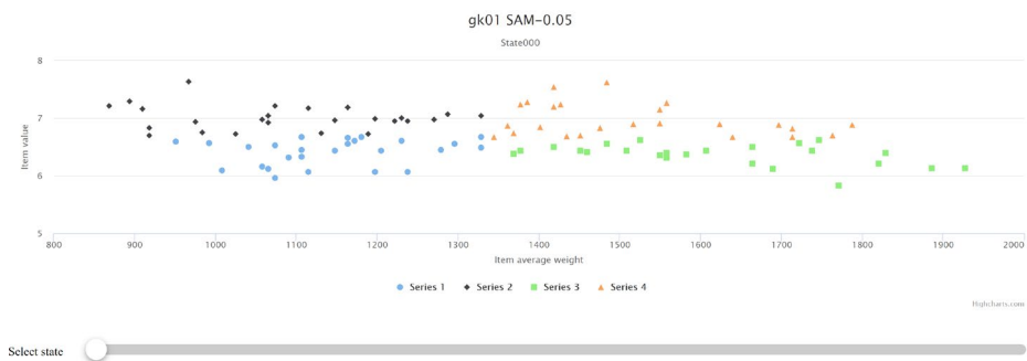
525 Fig. 12. Profit and weight distance effect for GK01 SAM-0.05 dataset initial state. Each series represent the division of each item's value and average weight into a quadrant based on the initial state. On the initial state, the division is clearly visible.
