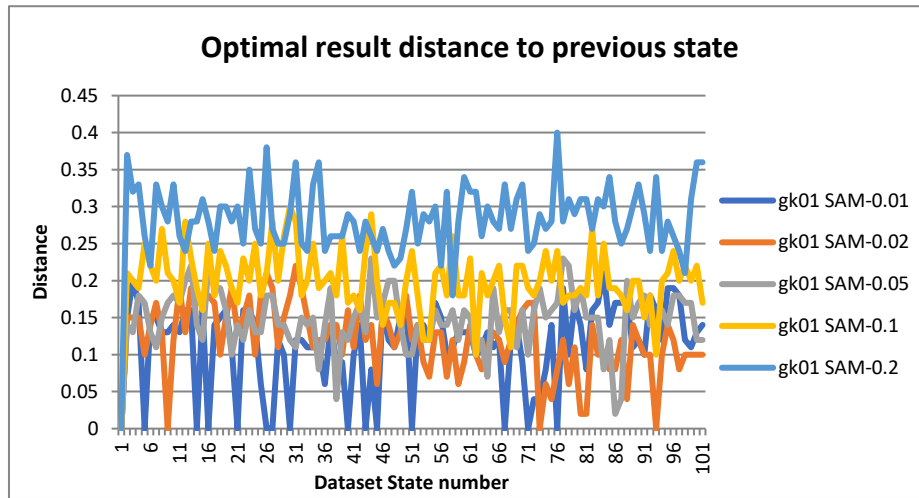
430 Fig. 9. Optimal result distance to the previous state for datasets generated from GK01
