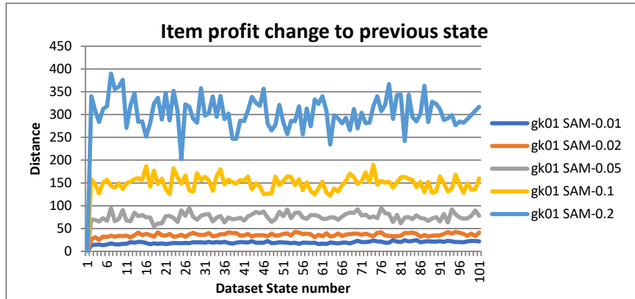
380 Fig. 5. Item profit change to the previous state for datasets generated from GK01
