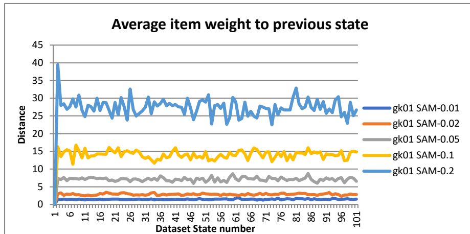
385 Fig. 6. Average item weight to the previous state for datasets generated from GK01
