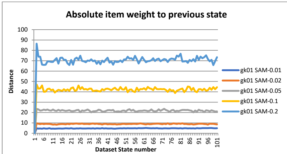
390 Fig. 7. Absolute item weight to the previous state for datasets generated from GK01
