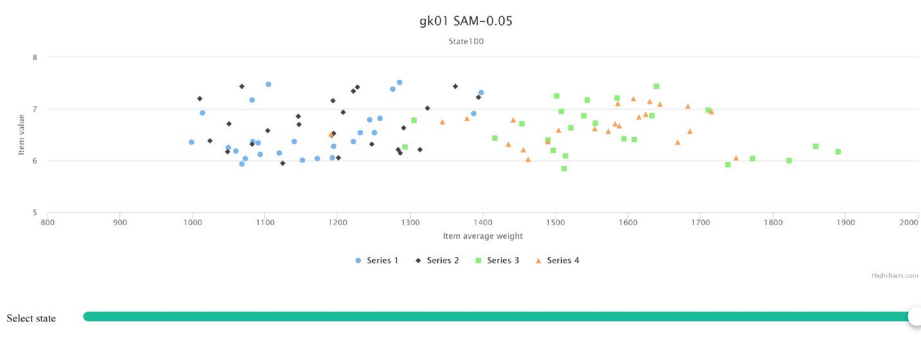
530 Fig. 13. Profit and weight distance effect for GK01 SAM-0.05 dataset last state. 531 Each series represent the division of each item’s value and average weight into a 532 quadrant based on the initial state. On the last state, items are significantly mixed 533 up.
