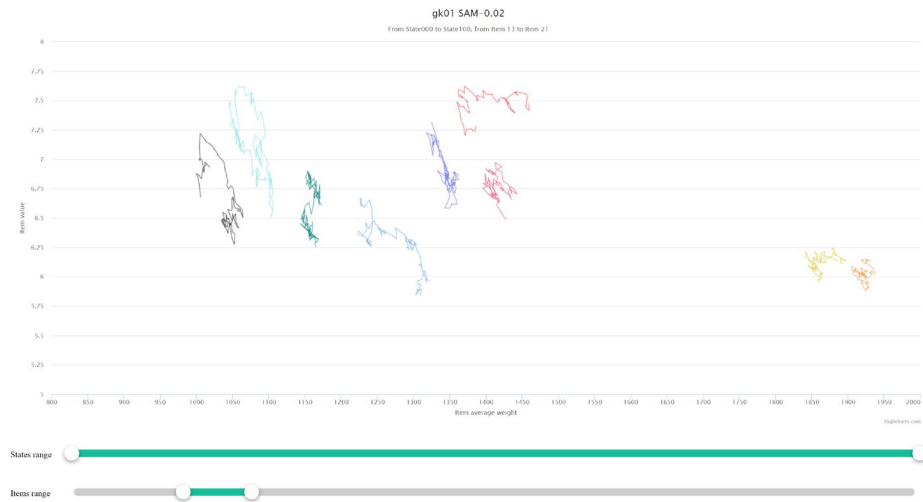
560 Fig. 16. Dynamic dataset constraint coverage effect, GK01 SAM-0.02 dataset, items range 13-21 inclusive.
