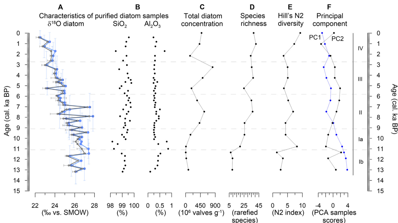
Fig. 4. Summary data for diatom samples from the Lake Emda Co1412 core: (A) measured \delta^{18}\text{O}_{\text{meas}} (grey line) shown with analytical errors and contamination-corrected \delta^{18}\text{O}_{\text{corr}} values of diatoms (blue line) shown with chronological errors and (B) SiO 2 and Al 2 O 3 concentrations in the purified diatom samples analysed by EDS and measured for \delta^{18}\text{O} ; (C) total diatom concentration, (D) species richness and (E) Hill's N2 diversity are plotted next to (F) the first two principal components (PC) sample scores (PC1 – blue line; PC2 – black line). (For interpretation of the references to color in this figure legend, the reader is referred to the Web version of this article.)
