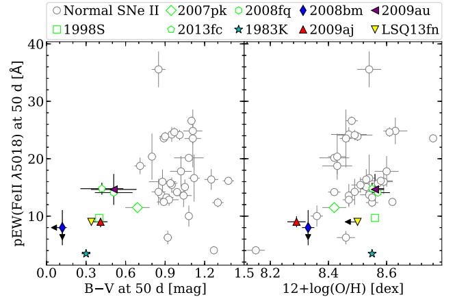
Figure 10. pEW of the Fe II \lambda 5018 line at 50 d since explosion as a function of the B - V colour (corrected for reddening) at the same epoch (left-hand side), and as a function of the oxygen abundance (right-hand side), showing the LLEV SNe II in our set (coloured filled symbols), the SNe II n /II from the literature (green empty symbols) and the normal SNe II in the A16 sample (grey empty circles). Arrows indicate upper limits.
