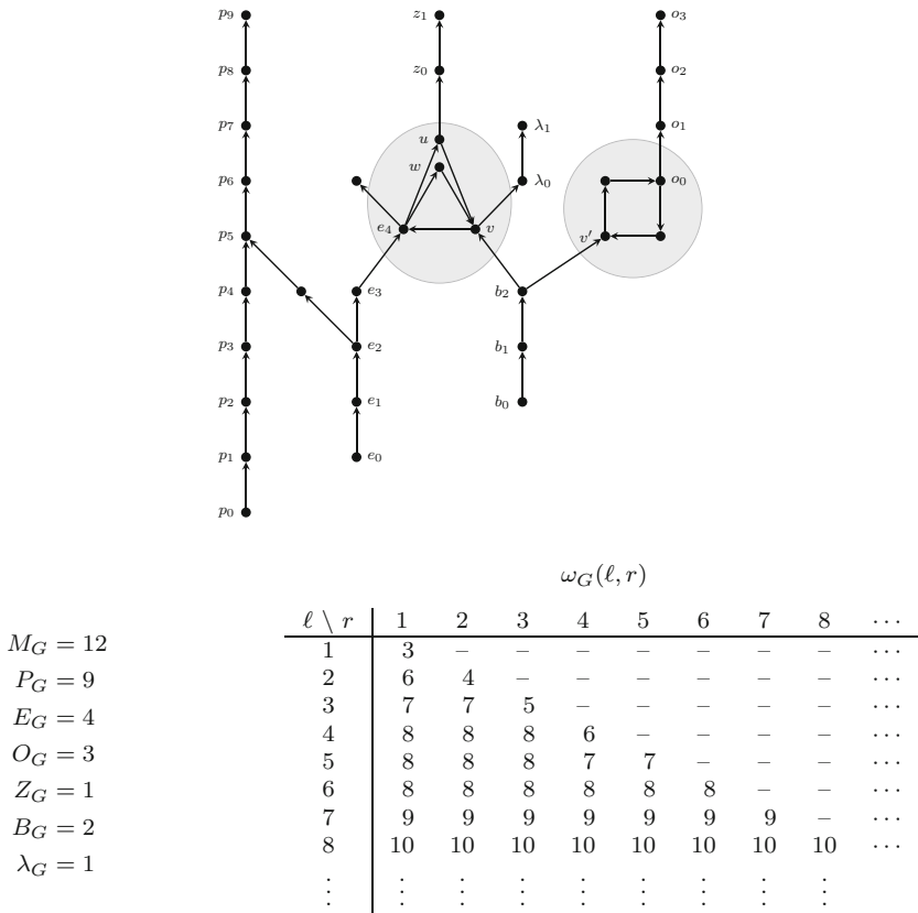
Fig. 1 Graph G and its structural parameters
