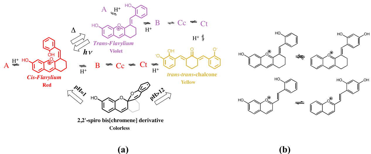
Scheme 14. Symmetric Spiro (II) Obtained from the Flavylium Cation (I)
