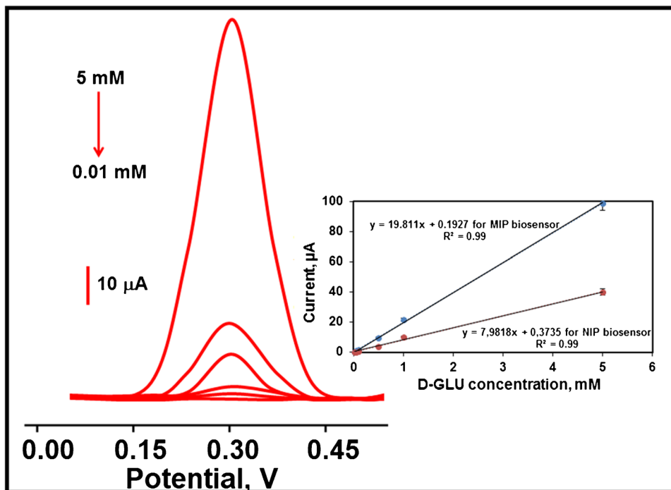
Fig. 5 Differential pulse voltammograms with different D-GLU amounts at MIP/TNO@NC/GCE in pH 7.0 of PBS (from 0.01 to 5.0 mM). Inset: D-GLU's calibration curves for MIP and NIP biosensors ( n=6 ) (parameters are frequency of 100 Hz, pulse amplitude of 25 mV, and scan increment of 5 mV)
