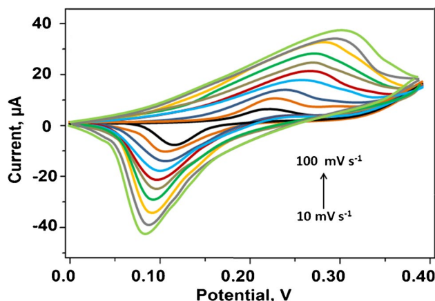
Fig. 6 Cyclic voltammograms curves at MIP/TNO@NC/GCE in pH 7.0 of PBS in 1.0 mM D-GLU solution at different scan rates (from 10 to 100 \text{mV s}^{-1} )
