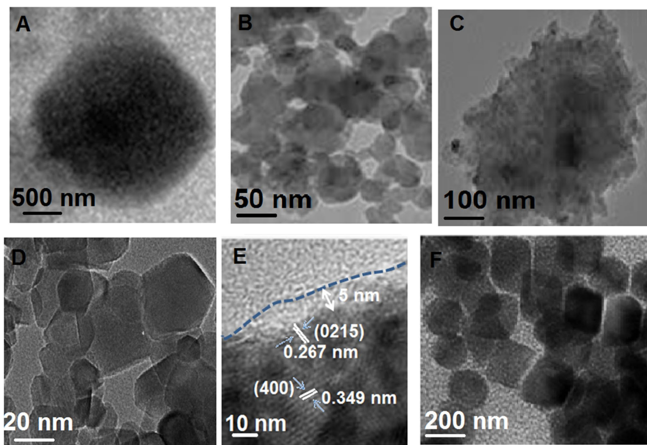
Fig. 1 TEM images of A bulk \text{Nb}_2\text{O}_5 , B ball-milled \text{Nb}_2\text{O}_5 , C \text{Nb}_2\text{O}_5 @PPy, D TNO@NC, E HRTEM image of TNO@NC, and F TEM image of pristine TNO
